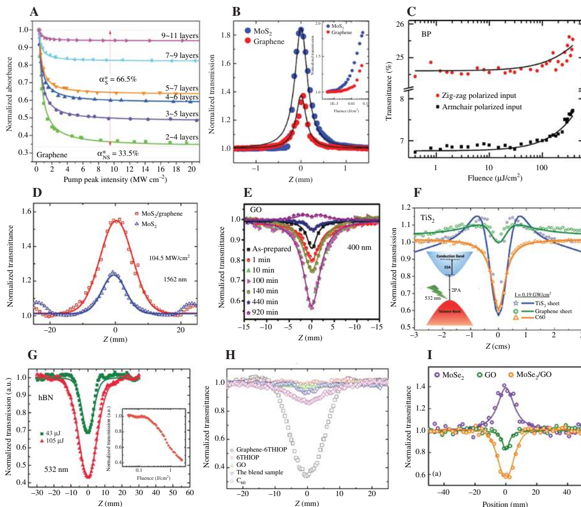
Figure 10: Nonlinear absorption in 2DLMs.
