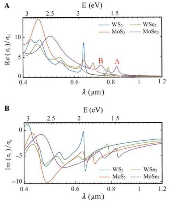
Figure 2: Dispersion of the complex sheet conductance of several TMDCs.
