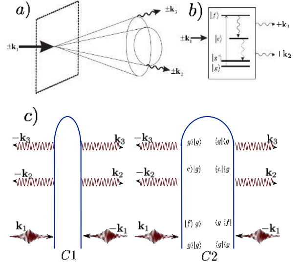
FIG. 31 Three wave process involving two quantum and one classical mode: (A) phase-matching condition; (B) molecular level scheme; (C) loop diagrams for the incoherent TPEF (C1) and coherent Type I PDC (C2)
