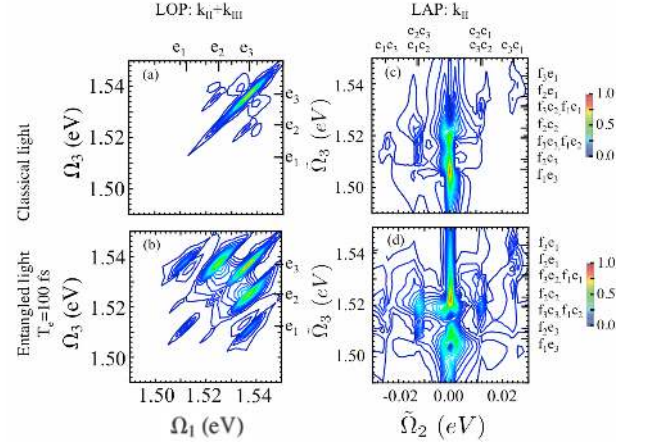
FIG. 18 (Color online) Left column: LOP signal S_{\mathbf{k}_{II}+\mathbf{k}_{III}}(\Omega_1, \tau_2 = 0, \Omega_3) for a molecular trimer with classical light Eq. (123) - (124) - (a), entangled light (125) with T_e = 100 fs - (b). Right: column: LAP signal S_{\mathbf{k}_{II}}(\tilde{\Omega}_1, t_2 = 0, \tilde{\Omega}_3) using classical light Eq. (119) - (c), entangled light with T_e = 100 fs, Eq. (128) - (d). Intraband dephasing \gamma_{ee'} = 1 meV. All other parameters are given in Section 5 of (Dorfman and Mukamel, 2014b).
