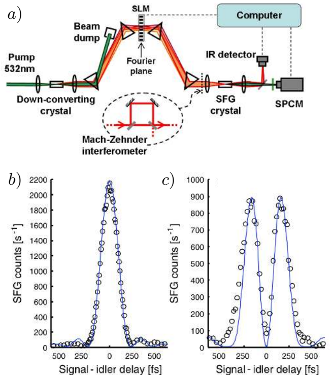
FIG. 5 (Color online) a) Experimental layout of the entangled photon shaper: A computer-controlled spatial light modulator (SLM) is used to manipulate the spectral phase of the entangled photons. The photon pairs are detected in the inverse process of PDC - sum frequency generation (SFG). The SFG photons are subsequently counted in a single-photon counting module. In order to demonstrate two-photon interference oscillations, a Mach-Zehnder interferometer is placed between the last prism and the SFG crystal. b) The SFG counts (circles) and the calculated second-order correlation function (line) of the unperturbed wavefunction as a function of the signal-idler delay. c) the same for the shaped wavefunction. Figure is taken from (Pe'er et al. , 2005).
