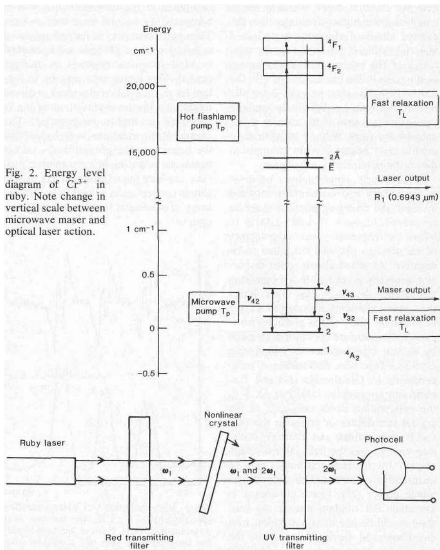
Fig. 3. Second harmonic generation of light.
