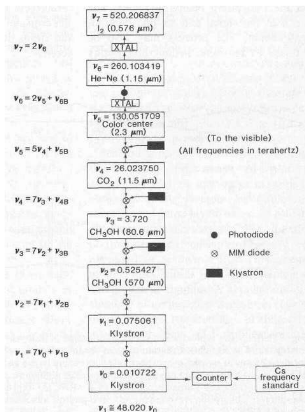
Fig. 6. Laser frequency synthesis chain (38).
