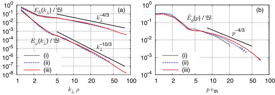
FIG. 3 (color online). Time-averaged normalized (a) wave-number (Fourier) spectra E_h(k_\perp)/2B and E_\varphi(k_\perp)/2B [cf. (9)], and (b) velocity-space (Hankel) spectrum \hat{E}_g(p)/2B for the runs indexed in Table I. Theoretically predicted slopes are given for comparison.
