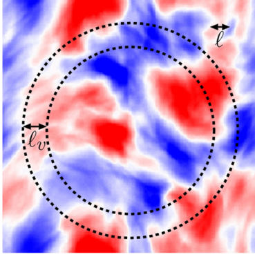
FIG. 1 (color online). Schematic view of the nonlinear phase mixing superimposed on the potential from the Run (iii) (see Table I) at t/\tau_{\text{init}} = 10 and the largest wavelength mode taken out. When the fluctuation scale \ell \lesssim \rho , the gyroaverage of the electric field induces a decorrelation of the distribution function at the velocity-space scale corresponding to the difference in Larmor radii \ell_v = \delta v/\Omega \sim \ell [see (7)].
