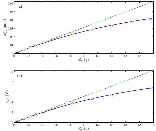
FIG. 6. (Color online) Comparison between linear theory (dotted line), nonlinear theory (solid line), and experimental measurements (O) at a fixed excitation frequency \Omega_e=545 Hz for the (a) mechanical response and (b) voltage across the resistive load.
