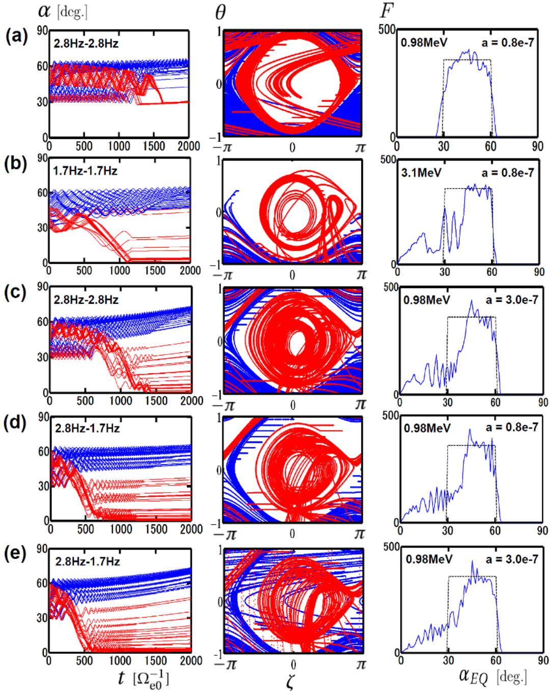
Figure 5. Time histories of pitch angles \alpha , trajectories of resonant electrons interacting with an EMIC wave packet with B_w = 0.009B_{EQ} in (\theta, \zeta) phase space, and distributions F of the resonant electrons in equatorial pitch angles \alpha_{EQ} after the interaction with the wave. The dashed lines indicate the initial distributions. (a) Case A: 0.98 MeV and constant \omega . (b) Case B: 3.1 MeV and constant \omega . (c) Case C: 0.98 MeV, constant \omega , and larger a . (d) Case D: 0.98 MeV and increasing \omega . (e) Case E: 0.98 MeV, increasing \omega ,
