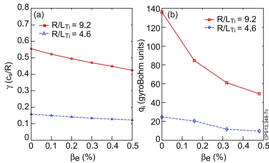
FIG. 3 (color online). Linear growth rates (a) and nonlinear ion heat fluxes (b) calculated in \beta_e and R/L_{Ti} scans based on discharge 66404 parameters. In the linear scan, k_y = 0.4 in units of 1/\rho_s . Runs included collisions, experimental geometry, two species, and assumed T_e/T_i = 1 .
