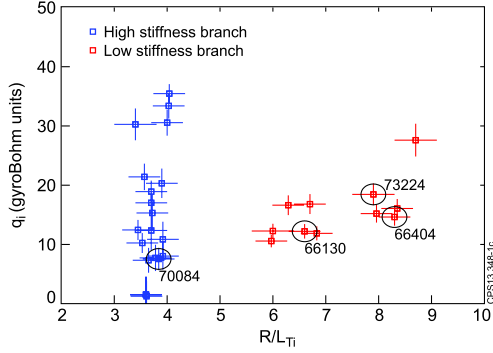
FIG. 1 (color online). Ion heat flux versus R/L_{Ti} , from JET data presented in Ref. [7] showing a separation between high and low stiffness regimes at \rho = 0.33 . The specific discharges studied in this Letter are circled.
