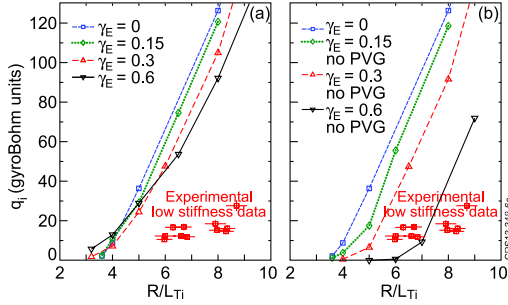
FIG. 2 (color online). Ion heat flux in nonlinear GENE R/L_{Ti} and \gamma_E scans based on discharge 70084 parameters at \rho = 0.33 ( q/\epsilon = 11.8 for circular geometry). \hat{s}/q = 0.2/1.3 throughout. Results are shown both including (a) and neglecting (b) PVG destabilization. All runs were electrostatic, collisionless, used circular geometry, and assumed T_e/T_i = 1 . The results are compared with the low stiffness data from Ref. [7].
