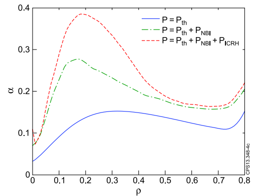
FIG. 4 (color online). The comparative influence of thermal and suprathreshold pressure components on \alpha for discharge 66404. Increased \alpha corresponds qualitatively to increased electromagnetic stabilization. The strong influence of suprathreshold pressure for \rho < 0.4 coincides with the measured low stiffness zone.
