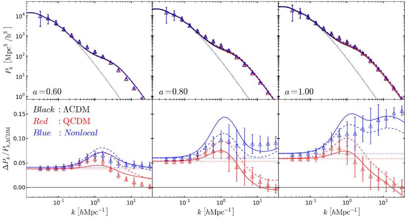
FIG. 7. The nonlinear matter power spectrum (upper panels) in the \Lambda\text{CDM} (black), QCDM (red) and R\Box^{-2}R (blue) models, at three epochs a = 0.6 , a = 0.8 and a = 1.0 , as labelled. The lower panels show the different w.r.t. \Lambda\text{CDM} . The symbols show the simulation results, where the errorbars show twice the variance across the five realizations of the initial conditions. The solid lines show the halo model prediction obtained using Eq. (25), with the best-fitting (q, p) parameters listed in Table IV. The dashed lines show the power spectrum when using the standard ST (q, p) = (0.75, 0.30) parameter values. The dotted lines show the result from linear perturbation theory. These lines are indistinguishable in the upper panels.
