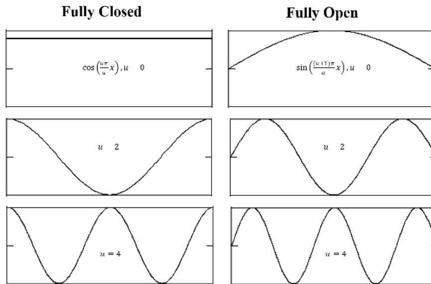
Figure 4. Acoustic mode shapes of the fully open and fully closed cavity boundaries.
