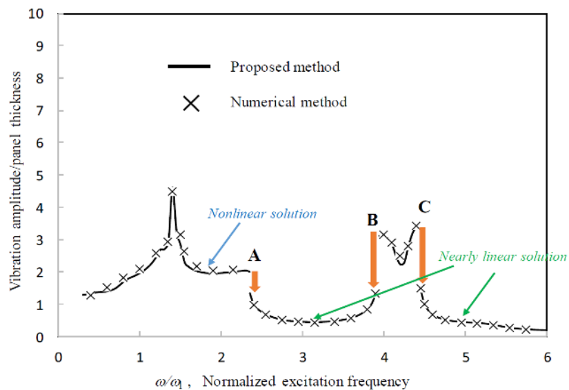
Figure 5. Comparison between the solutions obtained from the proposed method and numerical integration method [6] (number of structural modes = 2, number of acoustic modes = 4, l = 5a , \gamma = 2 , \theta = 0 ; the orange arrows represent the “jump phenomenon”; “A”, “B”, and “C” represent the particular points on the solution curve).
