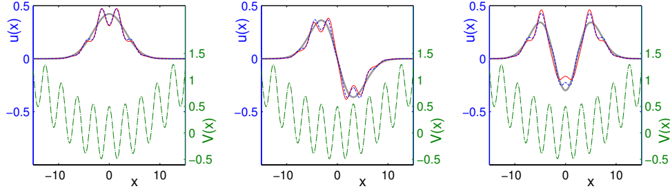
Figure 1. (Color online) The first three (left to right) eigenfunctions of the linear Schrödinger equation with the potential of Eq. (70). The thick gray solid line corresponds to the eigenfunction for the case of V_{\text{MT}}(x) , while the thin red solid and blue dashed lines correspond to the eigenfunction for V_{\text{MT}}(x) + V_{\text{OL}}(x) , as computed numerically and theoretically [see Eq. (78)], respectively. The full potential V_{\text{MT}}(x) + V_{\text{OL}}(x) (shifted for visibility, see scale on the right axis) is illustrated by the green dash-dotted line. The parameters used in this example correspond to V_0 = 0.5 and \Omega = 0.1 .
