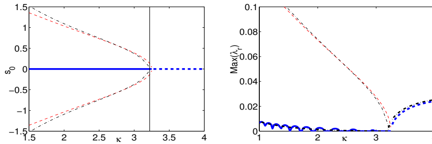
Figure 5. (Color online) An example of a subcritical pitchfork bifurcation in the parameter \kappa of the potential V(x) = x^2 \exp(-\kappa|x|) for fixed \epsilon = 0.2 in Eq. (107). The left panel shows the center of mass s_0 \equiv \xi of the dark soliton kink modes ( s_0 \neq 0 by dashed line, s_0 = 0 by thick solid and dashed lines). The theoretical predictions of s_0 based on Eq. (108) are shown by dash-dotted line. The vertical line gives the theoretical prediction for the bifurcation point \kappa = \kappa_0 = 3.21 . The right panel shows the real part of the unstable eigenvalues for the corresponding solutions, using the same symbolism as the left panel. The theoretical predictions of eigenvalues are shown by thick and thin dash-dotted lines, respectively for the branches with s_0 = 0 and s_0 \neq 0 . Notice that for the quartet of eigenvalues of the branch centered at the origin, the small jumps are due to the finite size of the computational domain (see Ref. [246] for details).
