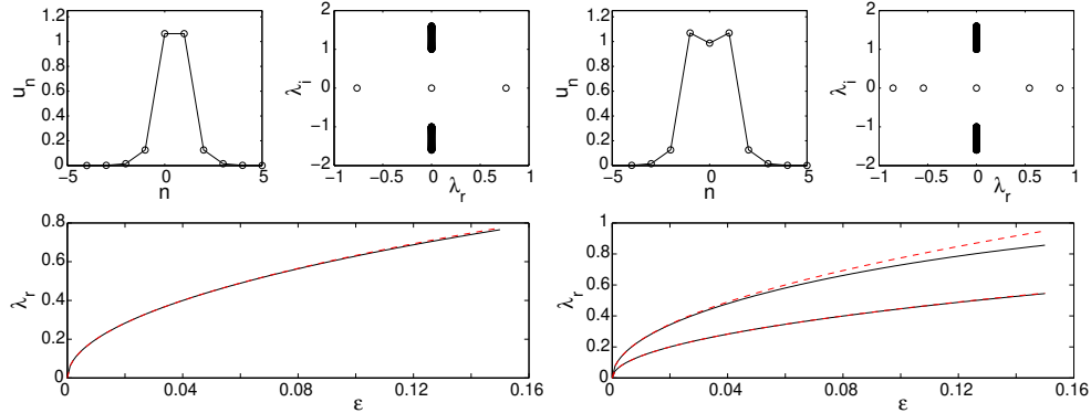
Figure 6. (Color online) A typical example of a two-site configuration is shown in the left panels of the figure, and a corresponding one of a three-site configuration in the right panels. The top panels show a solution (for a particular value of \epsilon ) and its corresponding spectral plane ( \lambda_r, \lambda_i ) of eigenvalues \lambda = \lambda_r + i\lambda_i , while the bottom ones show the dependence of the relevant real eigenvalues as a function of the inter-site coupling \epsilon obtained analytically (dashed/red lines) and numerically (solid/black lines).
