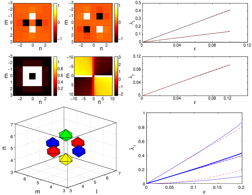
Figure 7. (Color online) The top panel shows a 2D S = 2 vortex configuration (left panels show its real and imaginary part -top- as well as amplitude and phase -bottom-) and its linear stability real and imaginary eigenvalues (right panels). Same thing in the bottom for a diamond 3D configuration (see the explanation for its phases in the text). The diamond configuration is shown using iso-level contours of different hues: blue/red (dark gray/gray in the black-and-white version) are positive/negative real iso-contours while the green/yellow (light gray/very light gray in the black-and-white version) correspond to positive/negative imaginary iso-contours. The theoretical predictions for the eigenvalues as a function of the coupling are shown by dashed line, while the full numerical results by solid ones. Partially reprinted from Ref. [280] with permission.
