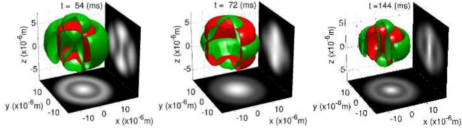
Figure 8. (Color online). Nonlinear dynamics of a binary 50:50 mixture of two spin states ( |1, -1\rangle and |2, 1\rangle ) of N = 375,000 Rb atoms. Each component is depicted by a contour slice at half of its corresponding maximal density. The bottom (side) projection corresponds to the z - ( x -) integrated density for the |1, -1\rangle component as it is observed in the laboratory experiments [322]. Please visit: http://www.rohan.sdsu.edu/~rcarrete/ [Publications] to view movies showing the inter-penetrating time evolution between the two components over a span of 220 ms. Reprinted from Ref. [322] with permission.
