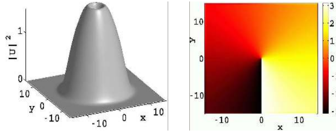
Figure 9. (Color online) Two-dimensional, singly charged ( S = 1 ), vortex inside a parabolic magnetic trap V(z) = \frac{1}{2}\Omega^2(x^2 + y^2) with \Omega = 0.2 . Depicted are the density (left) and the phase profile (right) for a chemical potential \mu = 2 .
