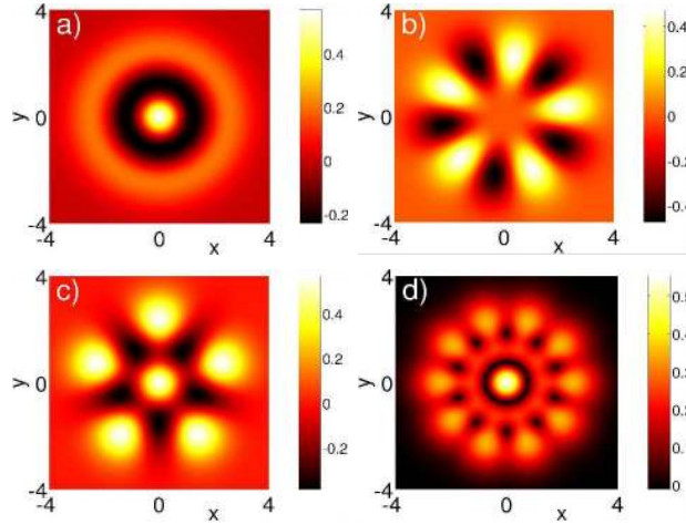
Figure 3. (Color online) A typical ring solution (top left), multipole solution (top right), soliton necklace (bottom left) and vortex necklace (bottom right) that can be obtained from the near-linear analysis of the 2D problem through Eqs. (90)–(92). Reprinted from Ref. [232] with permission.
