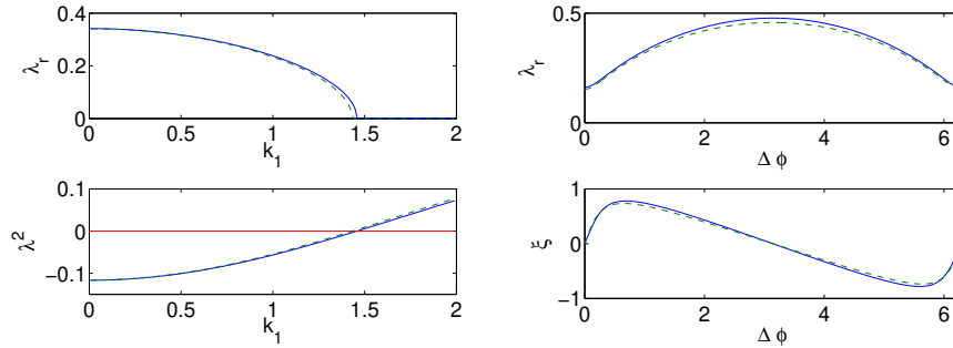
Figure 4. (Color online) Typical examples of the translational eigenvalue as obtained numerically (solid/blue line) versus the analytical prediction (dashed/green line). The linear and nonlinear potentials are: n_1(x) = A \cos(k_1 x) and n_2(x) = B \cos(k_2 x + \Delta\phi) . In the left panels we assume that A = B = 1 , and fix k_2 = 2\pi/5 and \Delta\phi = 0 and examine the relevant translational eigenvalue (its real part and its square) as a function of k_1 . Notice that there is a transition from instability to stability as k_1 is increased. In the right panels we select A = B = 1 and k_1 = k_2 = 2\pi/5 and vary \Delta\phi \in [0, 2\pi] . Notice that in the latter case the (critical point associated with the stationary) location of the solitary wave also changes with \Delta\phi and its theoretical and numerical values are also given (again in dashed and solid lines, respectively). Notice in all the cases the accuracy of the theoretical prediction.
