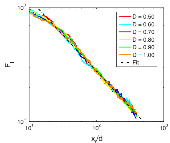
FIG. 8. (Color online) Force amplitude of the leading front of the delocalized wave as a function of its position x_f in the chain. For each curve, we average over ten configurations of the chain with disorder level D > D_c . As the wave propagates and after a short transient, the force amplitude decays as a power law with a coefficient of about 0.63, which is close to the theoretical prediction of \mu = 3/5 .
