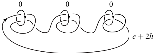
Figure 5: Kirby diagram for Q_{h,e} , shown when h = 3
