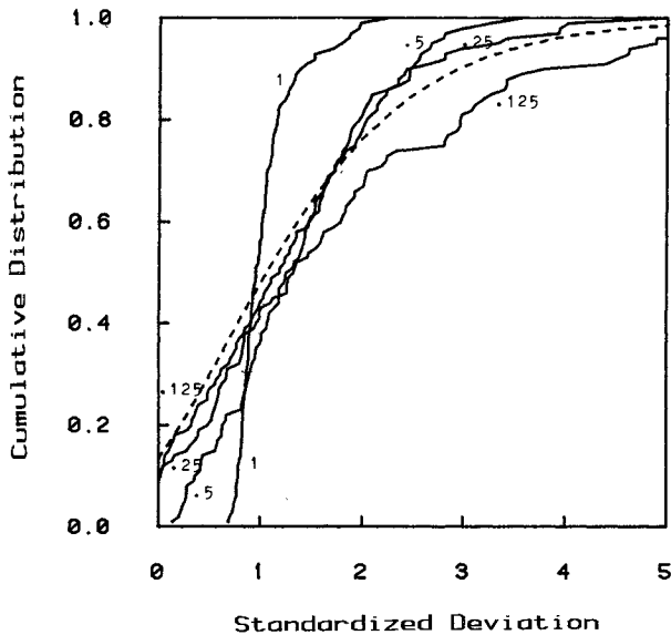
FIG. 4. EDF of maximal deviation as bandwidth b varies ( n = 200 , trials = 100). Short-dash = theoretical. Solid EDFs are b = 4.4835n^{-0.2} \times 1.0, \times 0.5, \times 0.25, and \times 0.125 . No censoring.
