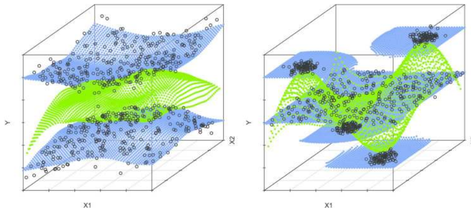
FIG. 9. Two examples for d = 2 . Modal regression estimates are shown in blue, and local regression in green.
