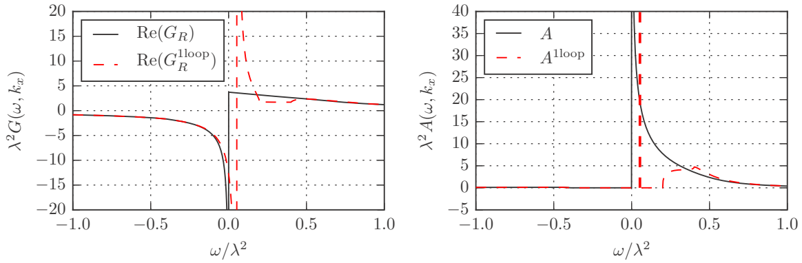
FIG. 8. The real and the imaginary part Green's function at the outer Fermi surface ( k_x = k_x^* \approx 0.4\lambda^2 and v = 0.5 ) as a function of \omega (solid line), and the one-loop truncated result (dashed). The spectral weight of the one-loop approximation is concentrated to a \delta function, whereas the spectral weight of the full result is spread in the power-law singularity.
