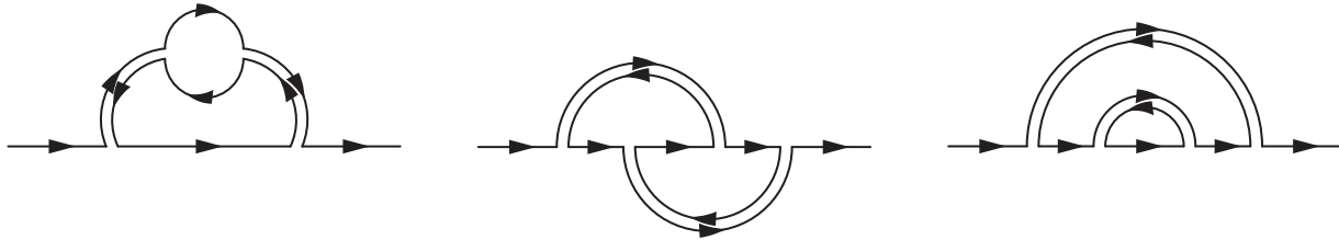
FIG. 2. The two-loop contributions to the fermion self-energy in theory in Eq. (3). The quenched limit where N_f \rightarrow 0 only suppresses the fermion loop contribution (a), whereas matrix large N limits, where the boson is a N \times N matrix \phi_i^j and the fermion a N -component vector \psi_i also suppress crossed diagrams of type (b). This is evident in double line notation of the same Feynman diagrams where the fermion is written as a single line (it has one index) and the matrix-valued boson as two lines (it has two indices). Indices have to match at interactions; each closed loop therefore corresponds to a sum over this index and gives a weight N to the diagram. We then see that the crossed diagram has no loops and is thus subdominant in N to other diagrams at the same order in the coupling constant.
