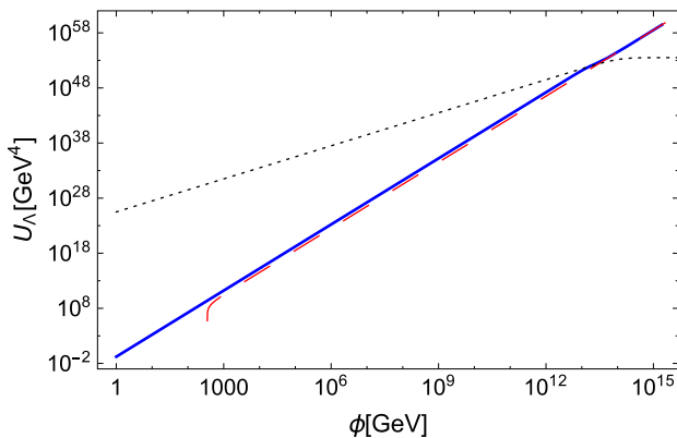
Fig. 2 Numerical solution of Eq. (13) for the bare potential U_\Lambda (blue solid line) for \Lambda = 10^{14} GeV. The IR physics is governed by a quartic Higgs potential (red dashed line) by construction. The black dotted curve shows the contribution of the scalar fluctuation induced part as well as the absolute value of the fermion induced part. As the difference of both contributions are hardly visible by eye in this double logarithmic plot, they appear as one line, indicating that both contributions almost compensate each other
