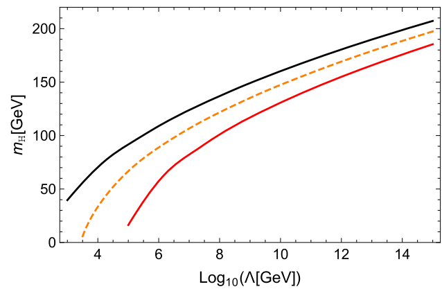
Fig. 1 Comparison of Higgs mass consistency bounds for different bare potentials. The black solid curve belongs to the conventional lower stability mass bound for quartic bare potentials. The orange dashed line is obtained from the lowest possible Higgs masses for the class of \phi^6 bare potentials with a unique minimum for the bare as well as the effective potential. The red solid line depicts the lower consistency mass bound for bare potentials given by Eq. (11) for a = 10^{-4} and \lambda_{2,\Lambda} = -0.18
