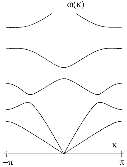
FIG. 1. Reciprocal electromagnetic spectrum of the three-layered periodic stack in Fig. 6 with \varphi=0 . The numerical set 1 from Eq. (82); F/A=1 .
