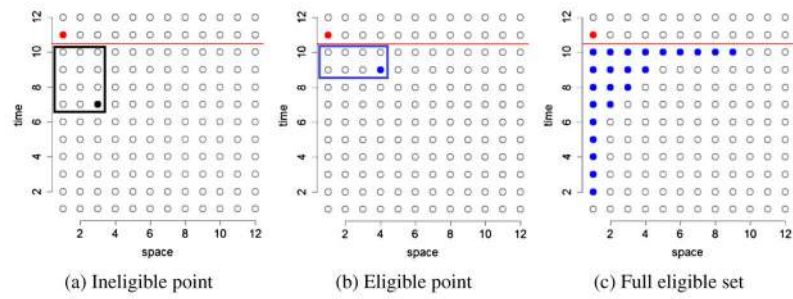
Fig. 3. Construction of eligible sets for finding nearest neighbor sets of size m = 9 : In figure (a) the black point is ineligible because the black rectangle contains more than m = 9 points. In figure (b) the blue point will belong to E(s_i, t_j) as the blue rectangle contains less than m = 9 points. Figure (c) shows the final eligible set obtained by repeating this algorithm for all points in the history set (below the red line).
