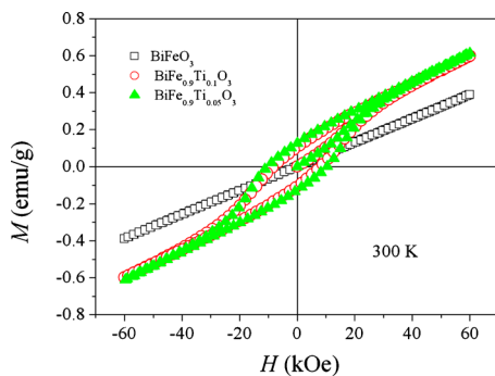
FIG. 6. (Color online) Magnetization hysteresis M - H loops of \text{BiFeO}_3 , \text{BiFe}_{0.9}\text{Ti}_{0.1}\text{O}_3 , and \text{BiFe}_{0.9}\text{Ti}_{0.05}\text{O}_3 ceramics.
