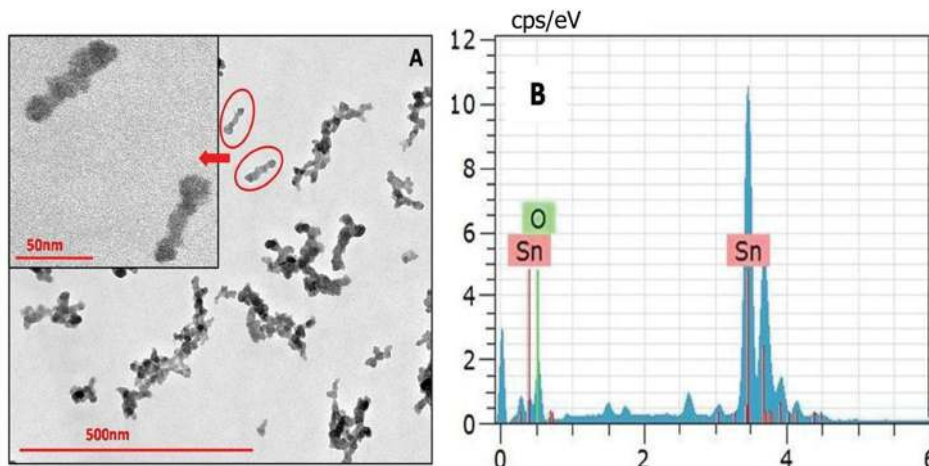
Fig. 6 (A) TEM image of \text{SnO}_2 NPs obtained via a solvothermal route in the relin matrix. (B) The EDX spectrum of the \text{SnO}_2 nanoparticles.
