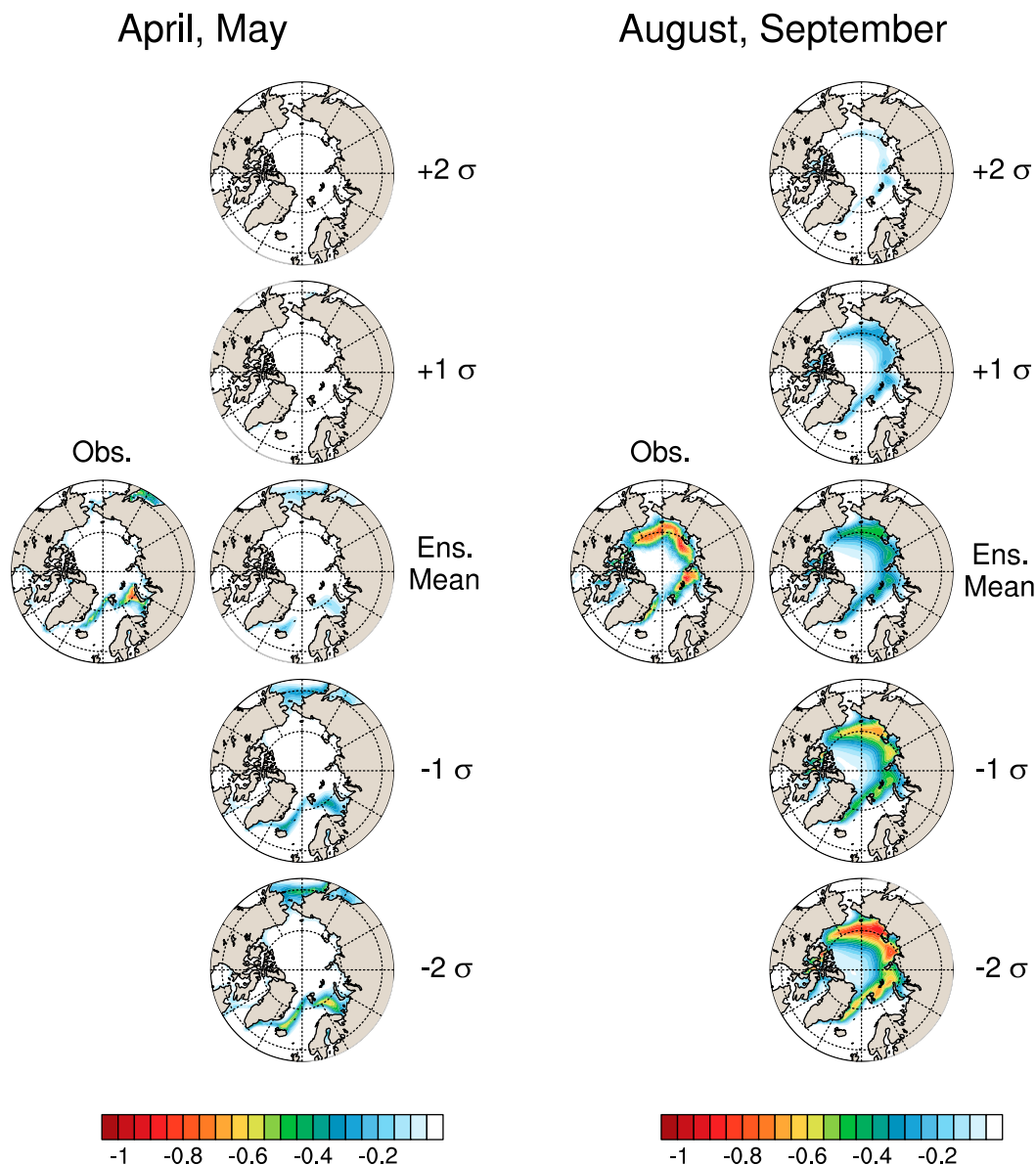
FIG. 7. Fifty-year changes in decadal means of Arctic sea ice fraction averaged over (left) April–May and (right) August–September from the HadISST dataset (“Obs.”) and ensemble mean (“Ens. Mean”) of the 40-member CESM-LE. The decades of interest are 1958–67 and 2008–17. Multiples of the standard deviation ( -2\sigma , -1\sigma , +1\sigma , and +2\sigma ) are calculated from the 40 members and then added to the ensemble mean to demonstrate the 95% range of expected changes.
