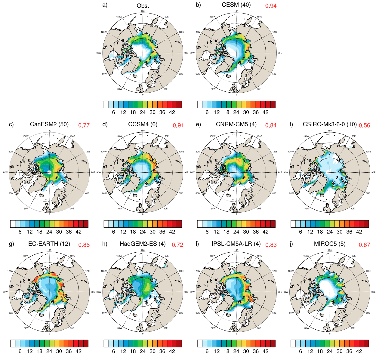
FIG. 2. Standard deviation of linearly detrended August–September sea ice concentration values 1958–2017 from (a) the HadISST observational dataset, (b) the 40 members of the CESM-LE, and (c)–(j) 8 CMIP5 models (CanESM2, CCSM4, CNRM-CM5, CSIRO Mk3.6.0, EC-EARTH, HadGEM2-ES, IPSL-CM5A-LR, and MIROC5). These are the CMIP5 models that have four or more ensemble members for the historical period, with the number of members displayed in parentheses after the model name. The pattern correlation score with observations is shown in red for each model.
