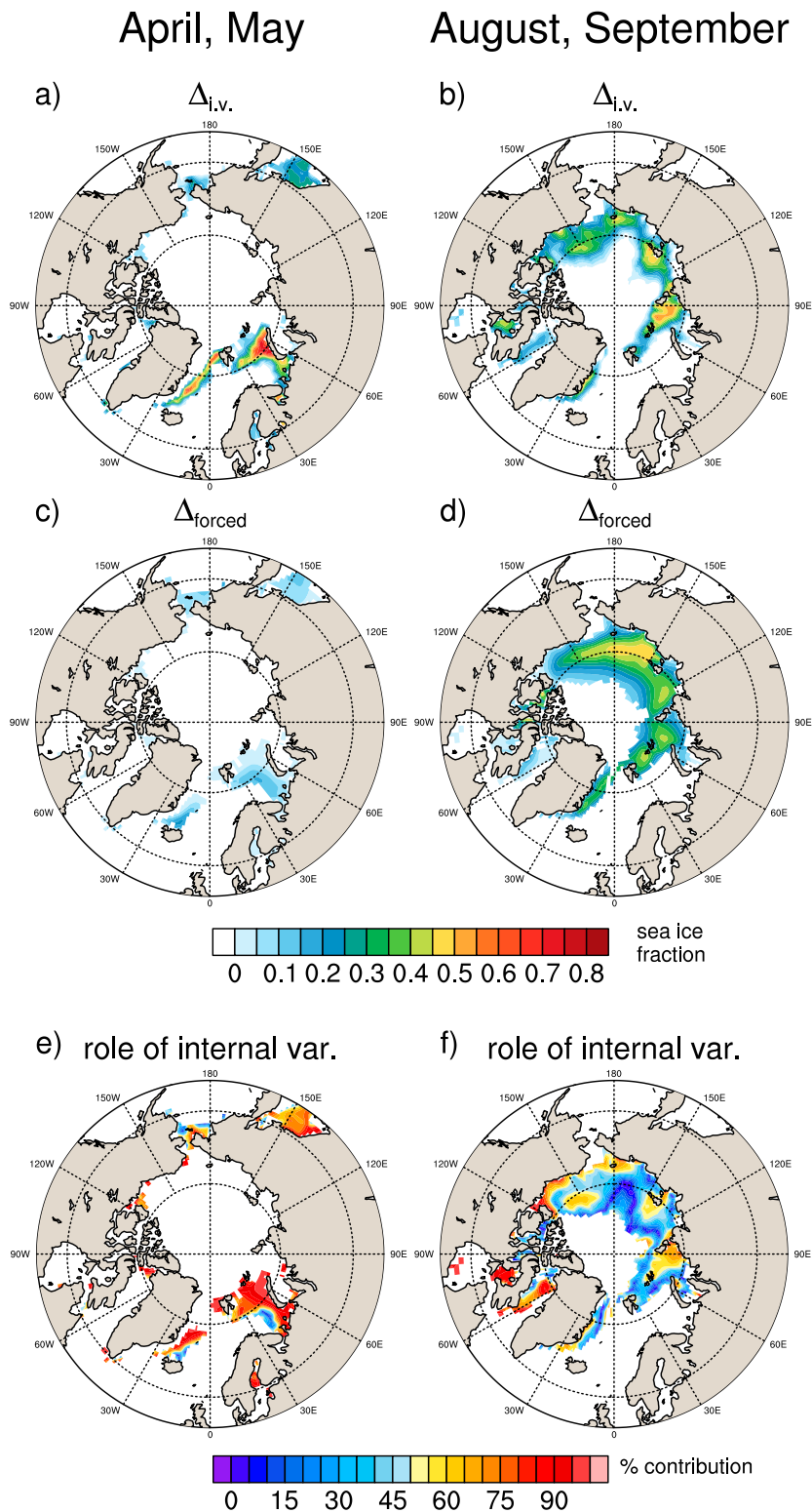
FIG. 8. For the 40 members of the CESM-LE, the contribution of (a),(b) internal variability and (c),(d) the forced response in (left) April–May and (right) August–September to the observed sea ice loss from 1958–67 to 2008–17 [shown in Fig. 7 (“Obs.”)], which is the sum of the top row and the middle row of this figure]. (e),(f) The percentage contribution of internal variability to the observed sea ice loss in each grid box, calculated as 100 \times [|\Delta_{iv}|/(\Delta_{iv} + \Delta_{forced})] . An example of the calculation for one grid box is given in Fig. 4.
