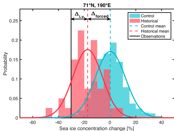
FIG. 4. The histograms are the distributions of 50-yr changes in decadal means from the 1800-yr CESM control run and the 40 members of the CESM-LE historical simulations for one gridbox ( 71^{\circ}\text{N} , 190^{\circ}\text{E} ). The contribution of internal variability in each grid box is calculated as 100 \times [\Delta_{i.v.}/(\Delta_{i.v.} + \Delta_{\text{forced}})] .
