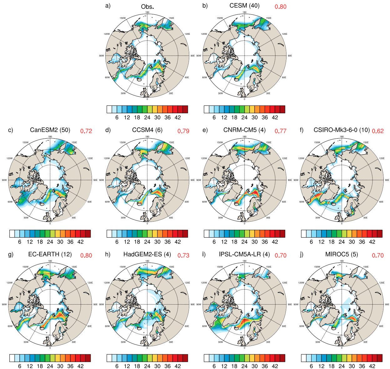
FIG. 3. As in Fig. 2, but for April–May.
