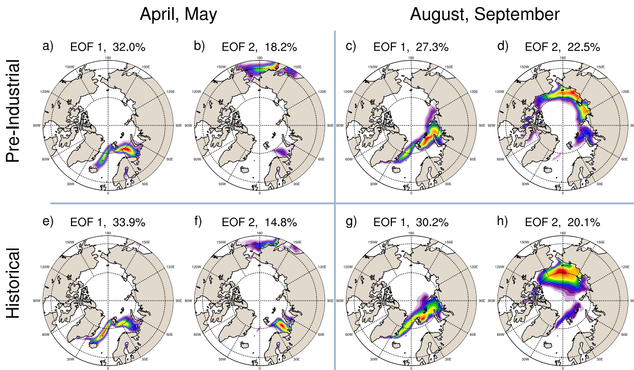
FIG. 10. The first two leading EOFs (normalized) of 50-yr changes in decadal means of Arctic sea ice fraction from (top) the CESM preindustrial control run and (bottom) from 1958–67 to 2008–17 from the CESM-LE. The control run provides 1741 overlapping 50-yr changes, and there are 40 independent 50-yr changes from the CESM-LE. We analyze the months (a),(b),(e),(f) April–May and (c),(d),(g),(h) August–September. The percentage of the total variance explained by the EOF is displayed, with the first two EOFs comprising one-half of the total variance. The remaining EOFs that are shown each account for less than 8% of the variance.
