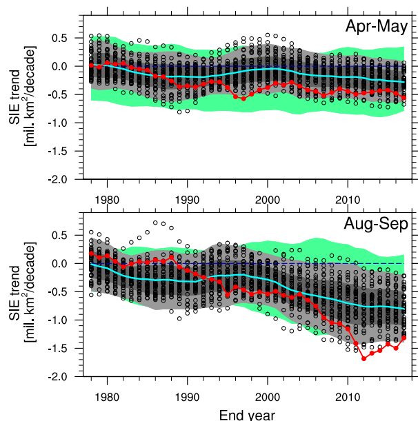
FIG. 6. Similar to Fig. 5, but for the 20-yr linear trends. The end year for these 20-yr trends ranges from 1978 to 2017. Trends for every pair of months in a year are shown in online supplemental Fig. S2.
