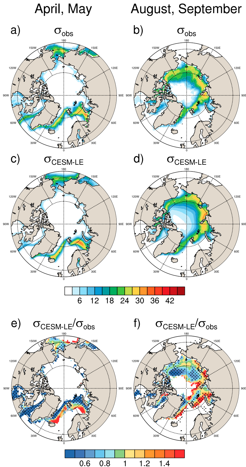
FIG. 1. Standard deviation of linearly detrended (left) April–May and (right) August–September sea ice fraction values over 1958–2017 from (a),(b) the HadISST observational dataset and (c),(d) the 40 members of the CESM-LE. (e),(f) The ratio of the two is shown for regions, and the stippling indicates differences that are significant using a false detection rate of 10%. Blue and red indicate that the CESM-LE under- and overestimates, respectively, the observed standard deviation.
