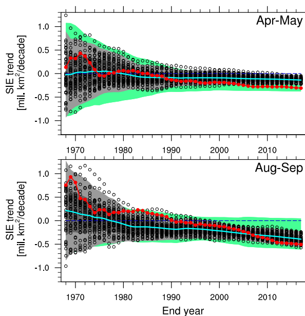
FIG. 5. Linear trends of Arctic sea ice extent that start from 1958 for the 40 members of the CESM-LE (black open circles), the CESM-LE ensemble mean (cyan line), and the observed value (red circles and line). The trends are of increasing lengths, with end years ranging from 1968 to 2017, reflecting trends of 10–50 yr. The dark-gray shading indicates values within 1 standard deviation of the ensemble mean, and the light-gray shading indicates within 2 standard deviations of the CESM ensemble mean. The green shading shows the 2\sigma envelope of trends found in the CMIP5 model ensemble. The blue dashed line shows the zero line. We divide the data into 2-month averages, with our focus in the study being April–May and August–September. Trends for every pair of months in a year are shown in online supplemental Fig. S1.
