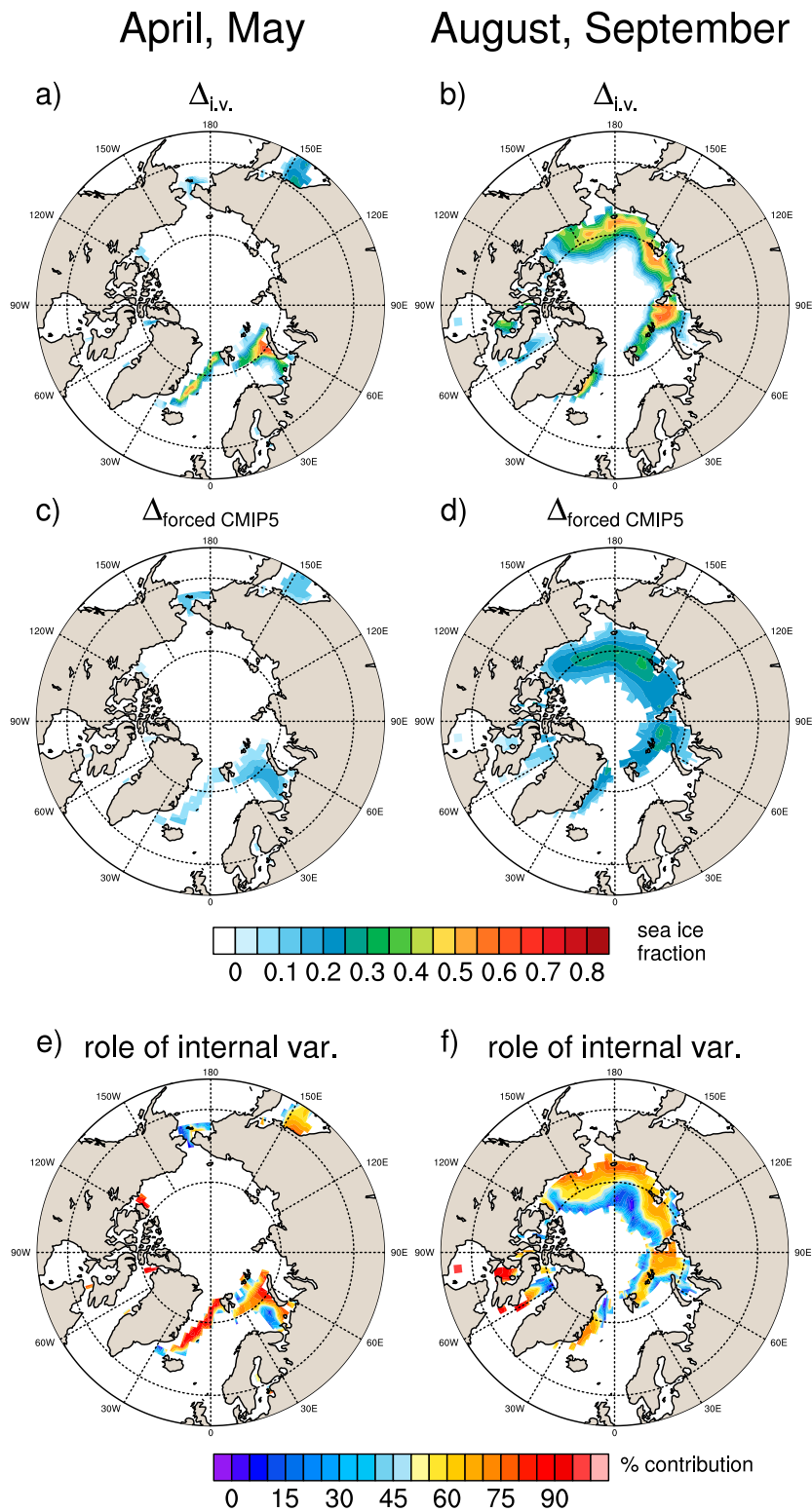
FIG. 9. As in Fig. 8, but based upon the CMIP5 ensemble mean change (averaged from 32 CMIP5 models).
