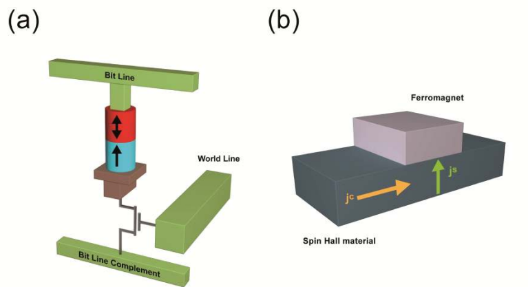
Figure 13. MRAMs based on spin-transfer and spin-orbit torque effects. (a) Schematic of the basic STT-MRAM unit showing the local magnetic element, whose state is controlled by a spin-polarized charge current flow. (b) Typical junction between a strong SOC-material giving rise to the spin Hall effect and a ferromagnet on which a pure spin current act to modulate/switch the magnetization (so-called spin-orbit torque effect).
