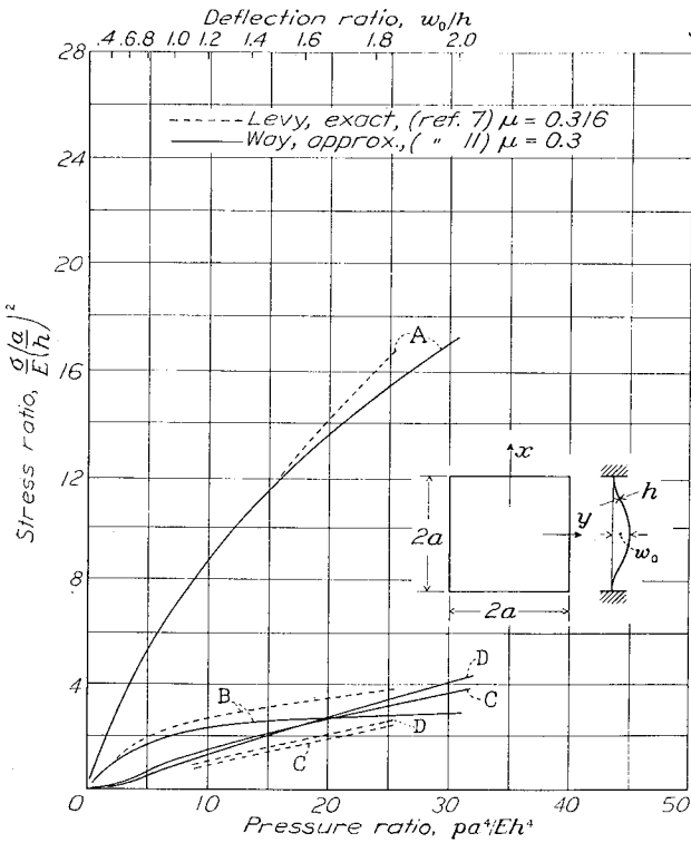
FIGURE 26.—Stress in a square plate with clamped edges. A, \frac{\sigma'_{xx}}{E} \left(\frac{a}{h}\right)^2 ; B, \frac{\sigma'_{xx}}{E} \left(\frac{a}{h}\right)^2 ; C, \frac{\sigma'_{xx}}{E} \left(\frac{a}{h}\right)^2 ; D, \frac{\sigma'_{xx}}{E} \left(\frac{a}{h}\right)^2 .
