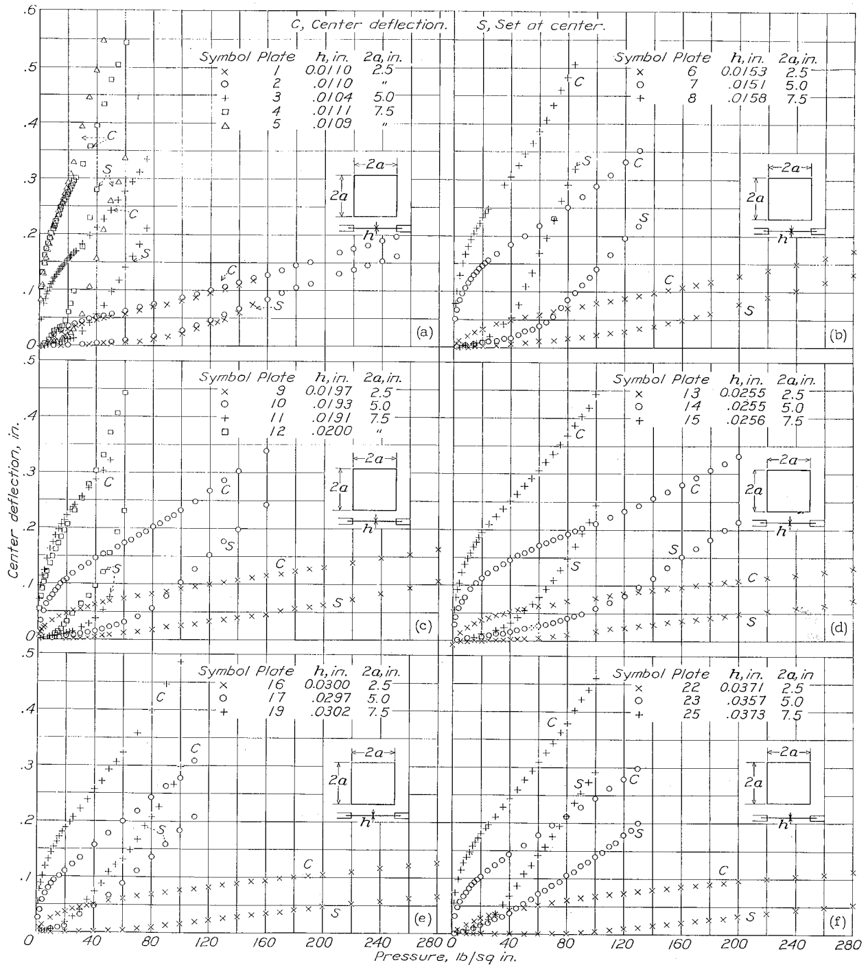
(a) Plates 1, 2, 3, 4, and 5. (b) Plates 6, 7, and 8. (c) Plates 9, 10, 11, and 12. (d) Plates 13, 14, and 15. (e) Plates 16, 17, and 19. (f) Plates 22, 23, and 25. FIGURE 11.—Deflection and set at center of 178-T aluminum-alloy plates with clamped edges.
