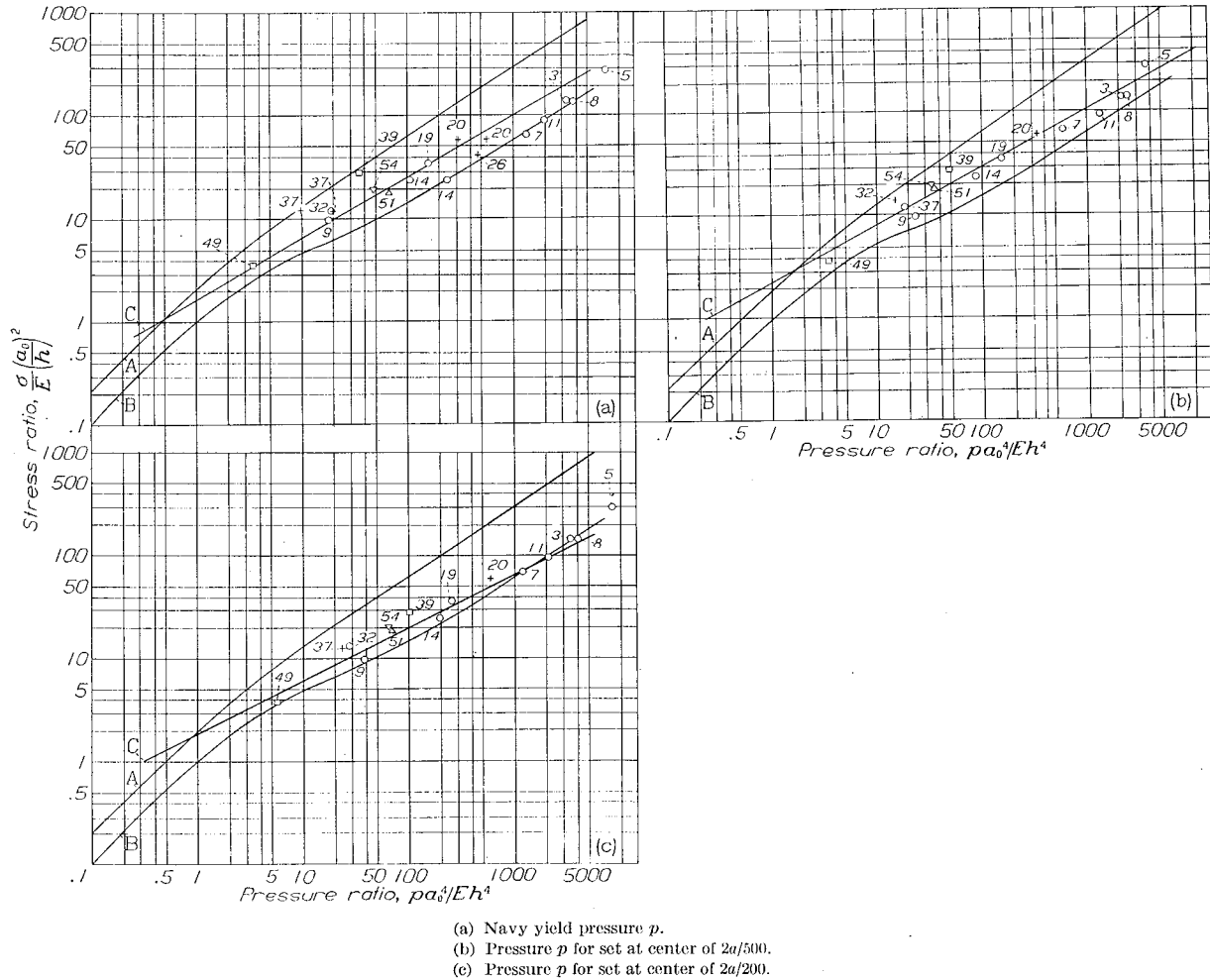
FIGURE 38.—Pressures for plates with clamped edges.
