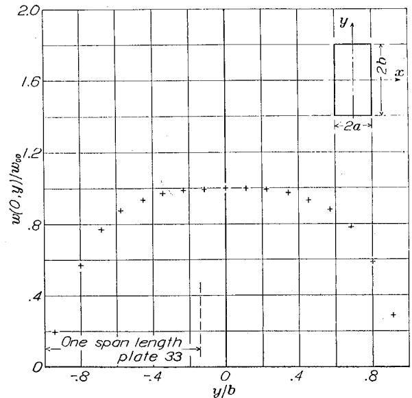
FIGURE 10.—Deflection curve along longitudinal center line of rectangular plate 33 (17S-T) with clamped edges. h , 0.0529 inch; 2a , 7.5 inches; 2b , 17.5 inches; w_0/h , 6.8; p , 50 pounds per square inch.
