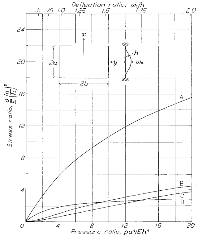
FIGURE 27.—Stress in a rectangular plate ( a/b=2/3 ) with clamped edges according to reference 11. Poisson's ratio, 0.3. A, \frac{\sigma''_{x_0}}{E} \left(\frac{a}{h}\right)^2 ; B, \frac{\sigma''_{x_e}}{E} \left(\frac{a}{h}\right)^2 ; C, \frac{\sigma'_{x_0}}{E} \left(\frac{a}{h}\right)^2 ; D, \frac{\sigma'_{x_e}}{E} \left(\frac{a}{h}\right)^2 .
