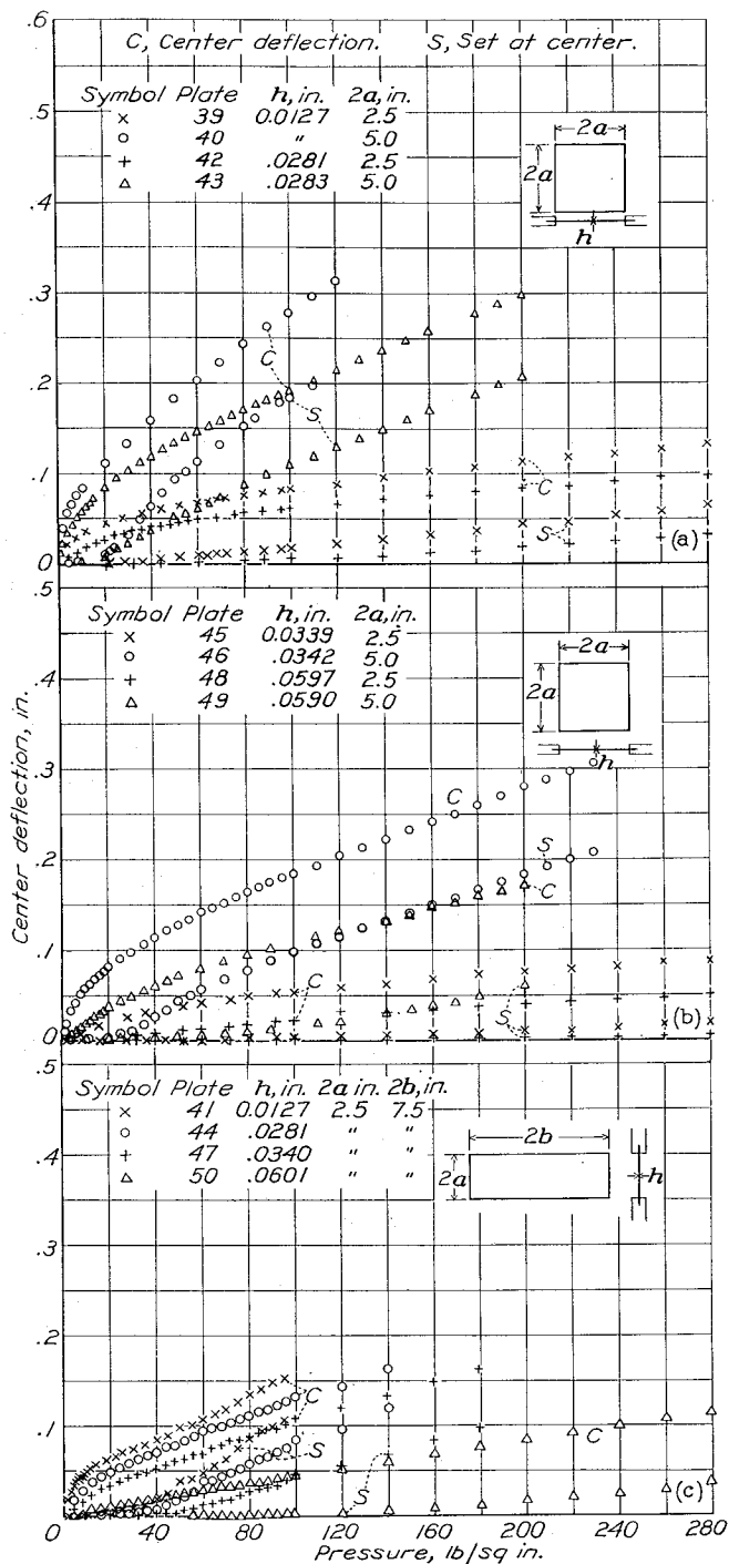
(a) Square plates 39, 40, 42, and 43. (b) Square plates 45, 46, 48, and 49. (c) Rectangular plates 41, 44, 47, and 50.
