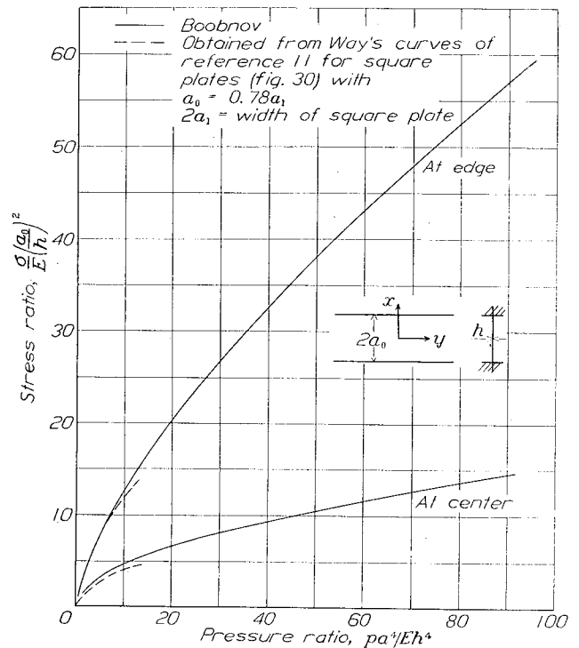
FIGURE 36.—Extreme-fiber stress in infinite plate strip ( a/b=0 ), clamped edges according to reference 12. Poisson's ratio, 0.3. p , pressure; E , Young's modulus.
