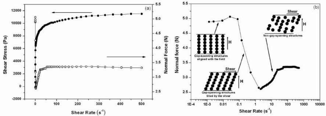
Figure 2. (a) Shear stress and normal force plotted as a function of shear rate; (b) relation between the different regimes of normal force and the expected microscopic particle structures. The solid (iron) volume fraction of the suspension is \Phi=10\% , and the applied field H=343\text{kA/m} .
