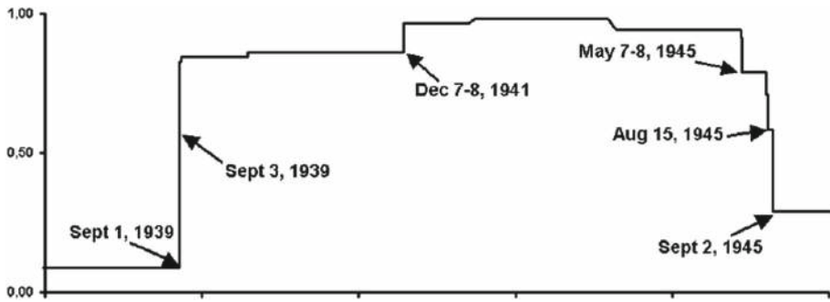
Fig. 2 Fuzzy set representing the time span of World War 2 [38]
