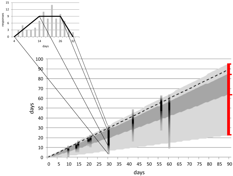
Fig. 9 Graphical representation of a normalisation model
