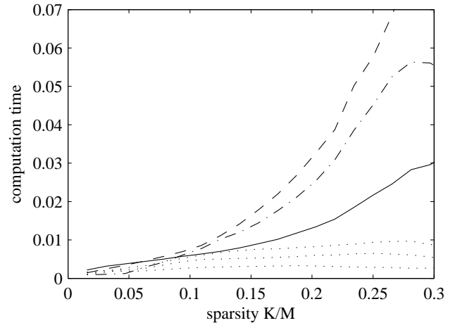
Fig. 5. Comparison between computation time for normalised IHT (solid), \ell_1 solution (dashed), CoSaMP using the pseudo inverse (dash-dotted) and CoSaMP using (from top to bottom) 9, 6 or 3 conjugate gradient iterations (dotted).
