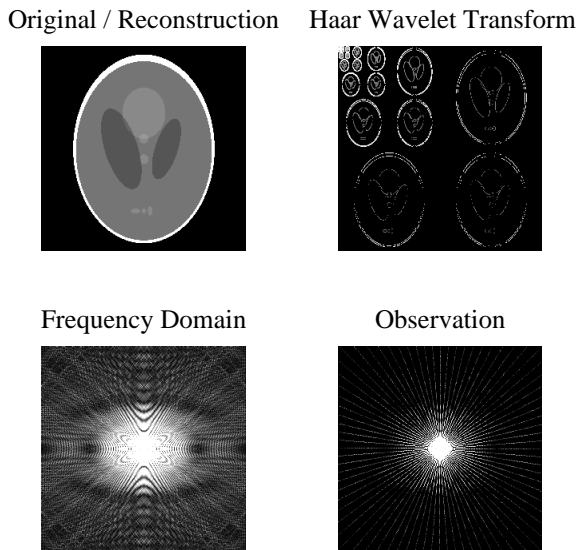
Fig. 8. Magnetic Resonance Imaging example using the Shepp-Logan Phantom. Original and reconstructed Phantom (top left), Haar wavelet representation (top right), Fourier domain representation (bottom left) and radial slices through the Fourier domain (bottom right).
