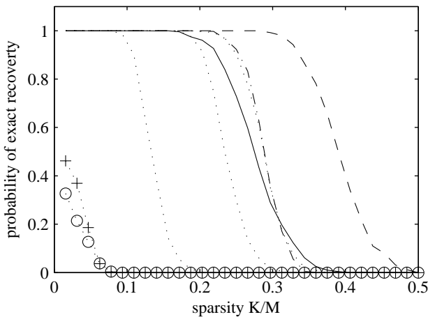
Fig. 4. Exact recovery performance where non-zero coefficients are 1. Comparison between normalised IHT (solid), \ell_1 solution (dashed), CoSaMP using the pseudo inverse (dash-dotted) and CoSaMP using (from left to right) 3, 6 or 9 conjugate gradient iterations (dotted). Also shown are the average cases in which the bound in subsection III-C did not violate the requirement in the algorithm (dotted o) and the cases in which the algorithm used \mu^{n+1} = \frac{\|\mathbf{g}_\Gamma\|_2^2}{\|\Phi_\Gamma \mathbf{g}_\Gamma\|_2^2} in all iterations (dotted +).
