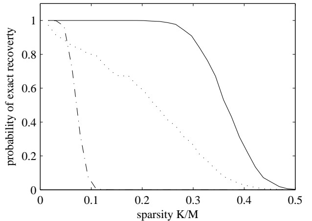
Fig. 2. Exact recovery performance. Comparison between the normalised IHT algorithm (solid), the un-modified algorithm where \|\Phi\|_2 = 1 (dotted) and the un-modified algorithm where \Phi has unit norm columns and the algorithm is stopped when the cost \|\mathbf{y} - \Phi\mathbf{x}\|_2 increases (dash-dotted).
