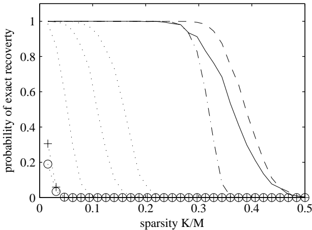
Fig. 3. Exact recovery performance where non-zero coefficients are Gaussian distributed. Comparison between normalised IHT (solid), \ell_1 solution (dashed), CoSaMP using the pseudo inverse (dash-dotted) and CoSaMP using (from left to right) 3, 6 or 9 conjugate gradient iterations (dotted). Also shown are the average cases in which the bound in subsection III-C did not violate the requirement in the algorithm (dotted o) and the cases in which the algorithm used \mu^{n+1} = \frac{\|\mathbf{g}_\Gamma\|_2^2}{\|\Phi_\Gamma \mathbf{g}_\Gamma\|_2^2} in all iterations (dotted +).
