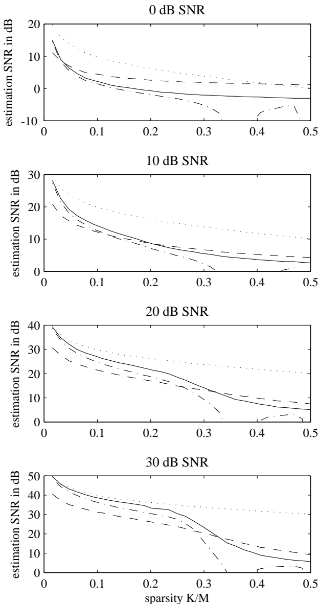
Fig. 6. Influence of observation noise. The observation was \mathbf{y} = \Phi\mathbf{x} + \mathbf{e} , where \mathbf{x} was K sparse. We compare normalised IHT (solid), \ell_1 solution (dashed) and CoSaMP (dash-dotted). Also shown is an oracle estimate that knows the location of the non-zero coefficients (dotted).
