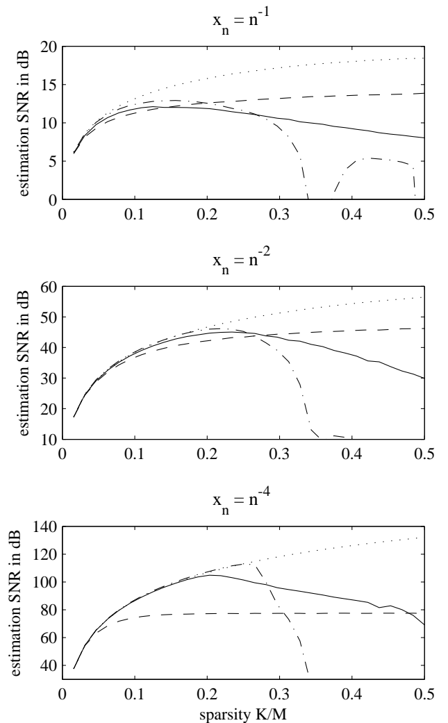
Fig. 7. Compressible signals. Here \mathbf{y} = \Phi\mathbf{x} , where \mathbf{x} was generated using x[n] = n^{-p} , for p \in \{1, 2, 4\} . We compare normalised IHT (solid), \ell_1 solution (dashed) and CoSaMP (dash-dotted). Also shown is an oracle estimate that knows the location of the largest K non-zero coefficients (dotted).
