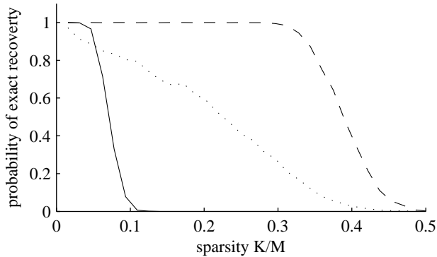
Fig. 1. Exact recovery performance. Comparison between \ell_1 minimisation (dashed), IHT_K where \|\Phi\|_2 = 1 (dotted) and IHT_K where \Phi has unit norm columns and the algorithm is stopped when the cost \|\mathbf{y} - \Phi\mathbf{x}\|_2 increases (solid).
