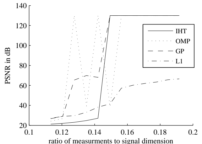
Fig. 9. Performance in recovering the Shepp-Logan phantom using radial line measurements. Ratio of measurements to signal dimension (x-axis) vs. peak signal to noise ratio (y-axis) (thresholded at 130 dB PSNR). Results are shown for normalised IHT, Orthogonal Matching Pursuit (OMP), 'Approximate' Conjugate Gradient Pursuit (GP) and \ell_1 optimisation (L1).
