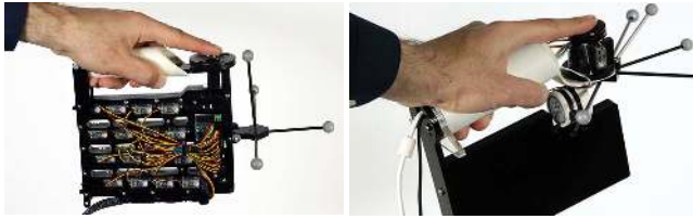
Figure 13: Devices used in the evaluation. (left) TextureTouch and (right) a modified NormalTouch controller, used for the NormalTouch interface, the VibroTactile interface (using an Xbox vibration motor), and the VisualOnly interface that tracked the user’s finger without haptic feedback.
