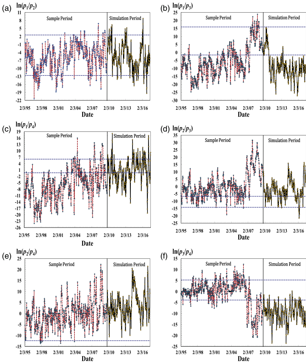
Figure 3. Time-series plots of natural logarithms of sample (dashed line) and bootstrap simulated (solid line) regional relative prices for OSB. Dashed horizontal lines denote approximate transactions cost bands
