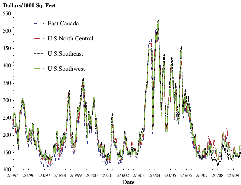
Figure 2. Regional weekly OSB prices, 1995–2009
