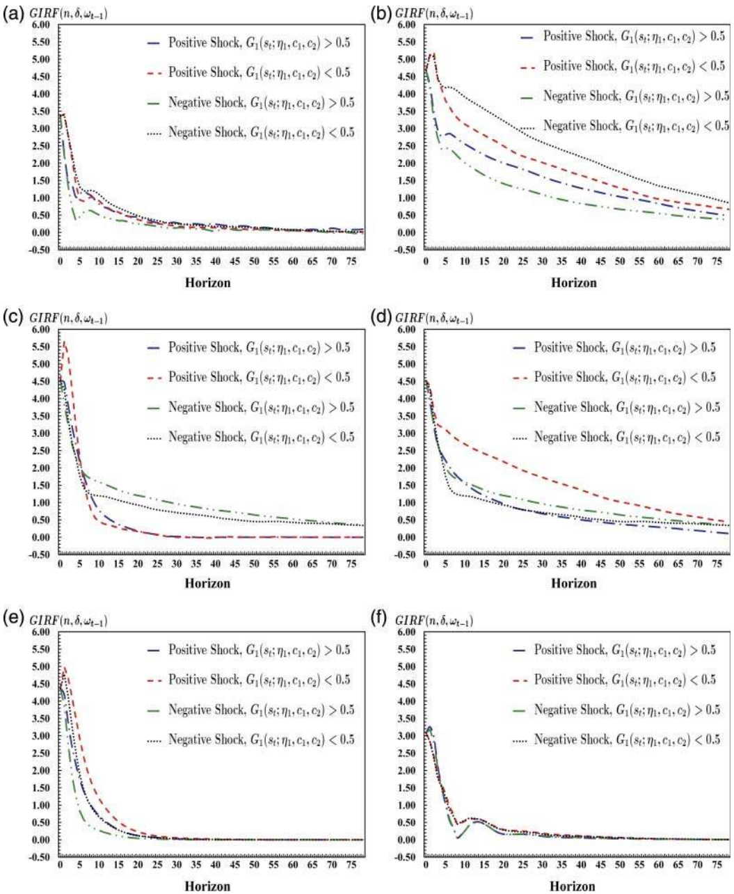
Figure 5. Estimated generalized impulse response functions for six regional OSB price relationships
