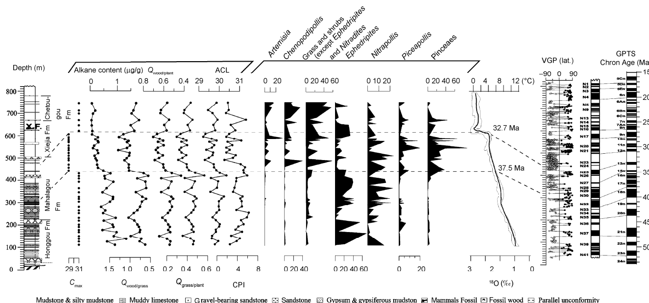
Figure 2 Time series of n -alkane proxies and pollen diagram showing abundance (%) of major floral components (detailed results are presented in another article 2) ) vs. stable isotope marine records. Age model from Dai [25]. Alkanes content ( \mu\text{g/g} ) = C_{27} + C_{29} + C_{31} + C_{33} ; Q_{\text{wood/grass}} = C_{27}/C_{31} ; Q_{\text{grass/plant}} = C_{31}/(C_{27} + C_{29} + C_{31}) ; Q_{\text{wood/plant}} = (C_{27} + C_{29})/(C_{27} + C_{29} + C_{31}) ; \text{CPI} = [(C_{25} + C_{27} + C_{29} + C_{31} + C_{33}) / (C_{24} + C_{26} + C_{28} + C_{30} + C_{32}) + (C_{25} + C_{27} + C_{29} + C_{31} + C_{33}) / (C_{26} + C_{28} + C_{30} + C_{32} + C_{34})] / 2 ; \text{ACL} = (27 \times C_{27} + 29 \times C_{29} + 31 \times C_{31} + 33 \times C_{33}) / (C_{27} + C_{29} + C_{31} + C_{33}) .
