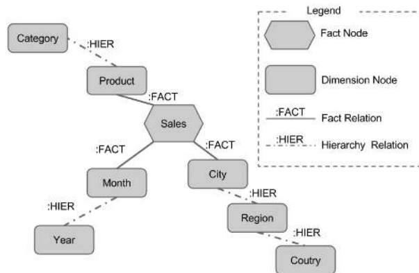
Figure 4: Modelling cubes and dimensions in a NoSQL Graph (Neo4J)
