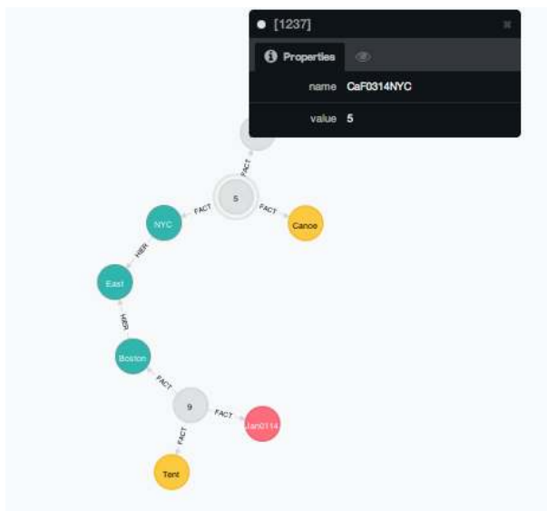
Figure 10: A Slice Operation over the NoSQL Graph Cube in Neo4j
