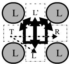
Fig. 5b Final make-up routing of a local S box
