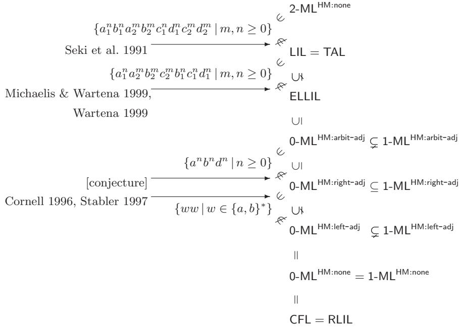
Figure 3: Schematic overview of our results. 10,11
