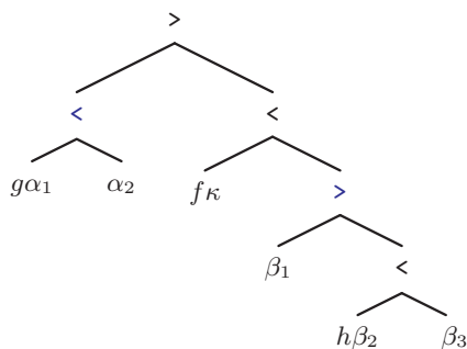
Figure 4: A typical (minimalist) expression. 14
