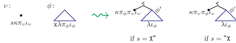
Figure 7: merge(v, \phi) — strong selection.
