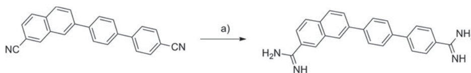
Scheme 3. Synthesis of an aromatic diamidine using LiN(TMS) 2 .
