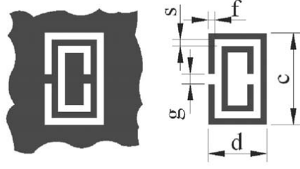
Figure 1. Geometries of the CSRRs and the SRRs, grey zones represent the metallization.
