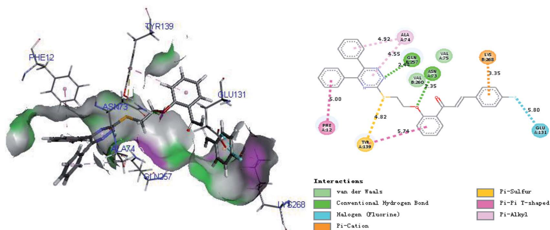
Fig. 5 The binding mode of compound 4l docked with TMV-CP.
