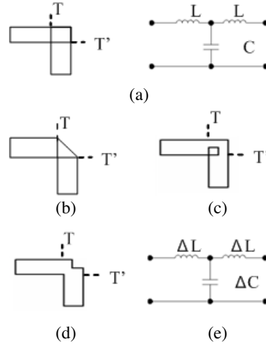
Figure 3. Various type of microstrip bending techniques, (a) 90° bend and its equivalent circuit, (b) 45° mitered, (c) inner cutoff, (d) outer cutoff and (e) their equivalent circuit.
