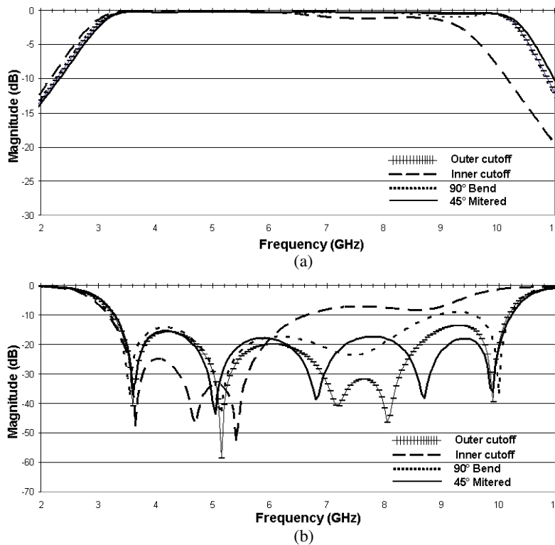
Figure 5. Simulated frequency response of “Butterfly” shape microstrip filter with four different types of bending, (a) insertion loss ( S_{21} ) and (b) return loss ( S_{11} ).
