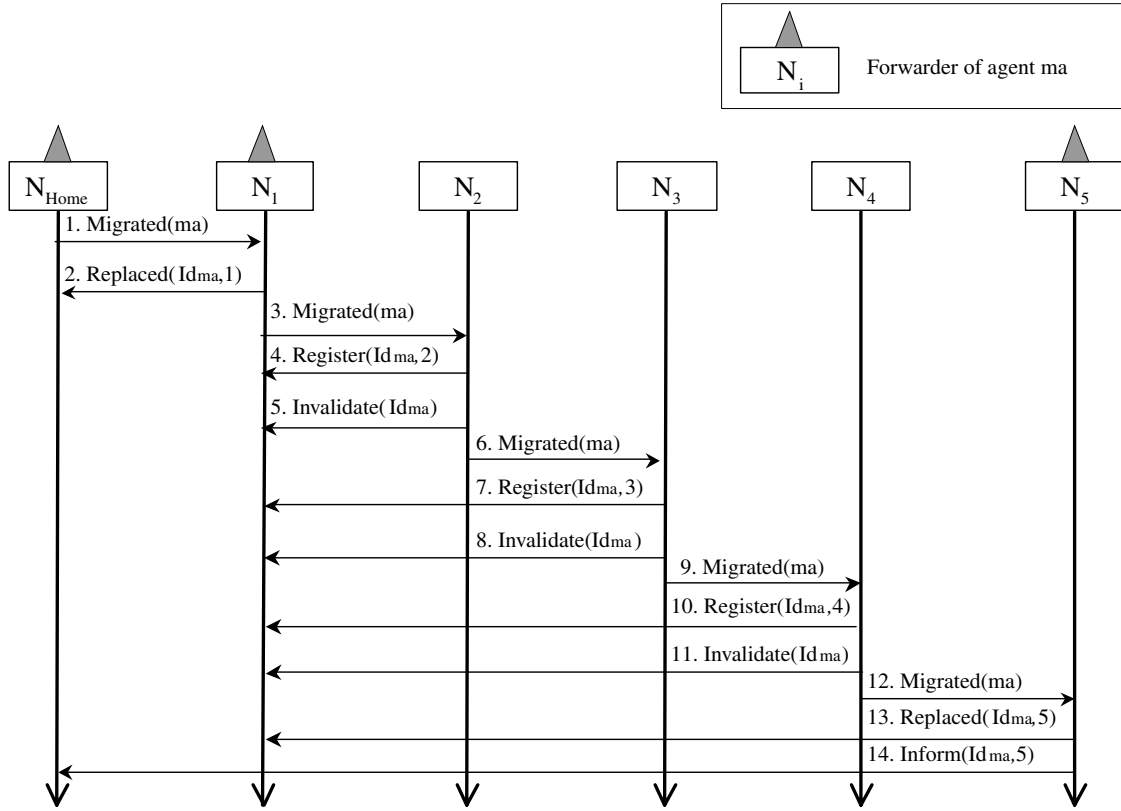
Fig. 5. An execution of our proposed directory service algorithm for an agent ma during its multi-node movement.
