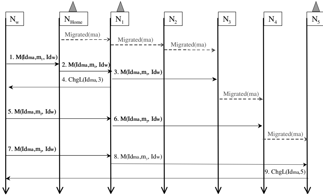
Fig. 8. An execution of reliably forwarding messages from their source agent \gamma to their target agent ma during its multi-node movement.
