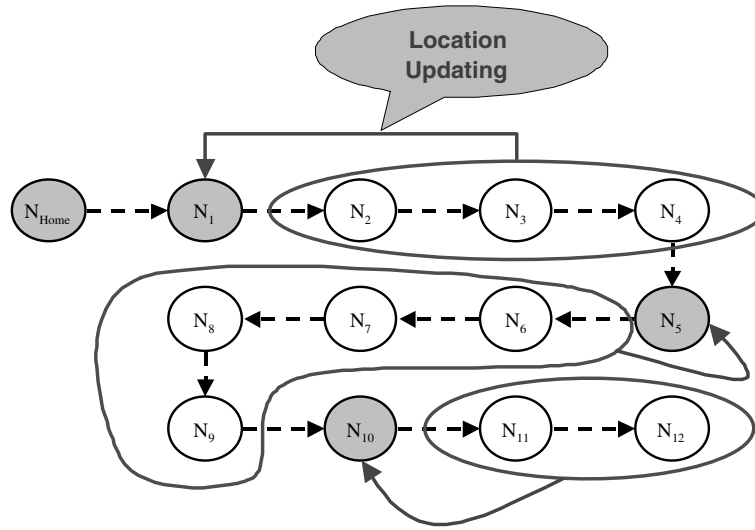
Fig. 4. Our scalable mechanism.
