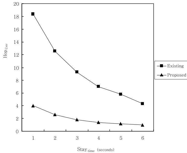
Fig. 11. Hop_{Cntr} vs. Stay_{time} .
