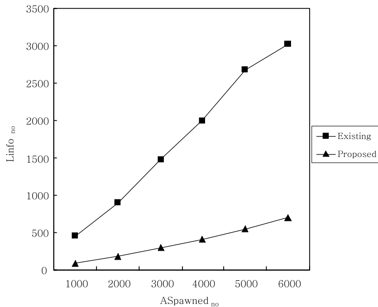
Fig. 12. LInfo_{no} vs. ASpawned_{no} .
