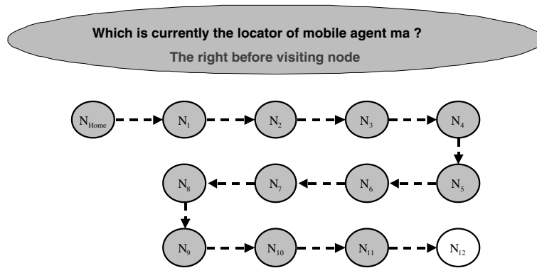
Fig. 3. Forwarding pointer-based mechanism.
