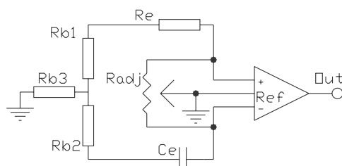
Figure 5. Input circuit of the operational amplifier used in the filter electrode setup using only two electrodes. The adjustable resistor R_{adj} balances the potential instead of using a third electrode as a reference.
