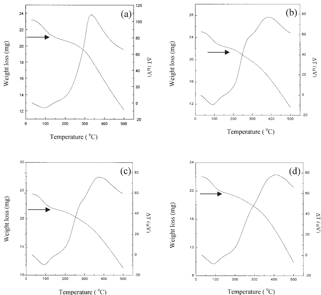
Figure 4 TGA/DTA tracings of (a) PANI-0, (b) PANI-2, (c) PANI-5, and (d) PANI-10 nanocomposites.
