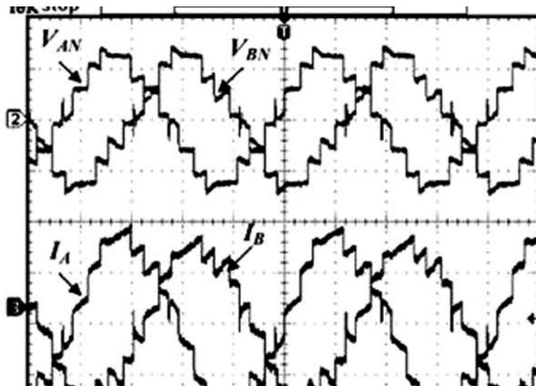
Figure 2. Test modulation.
