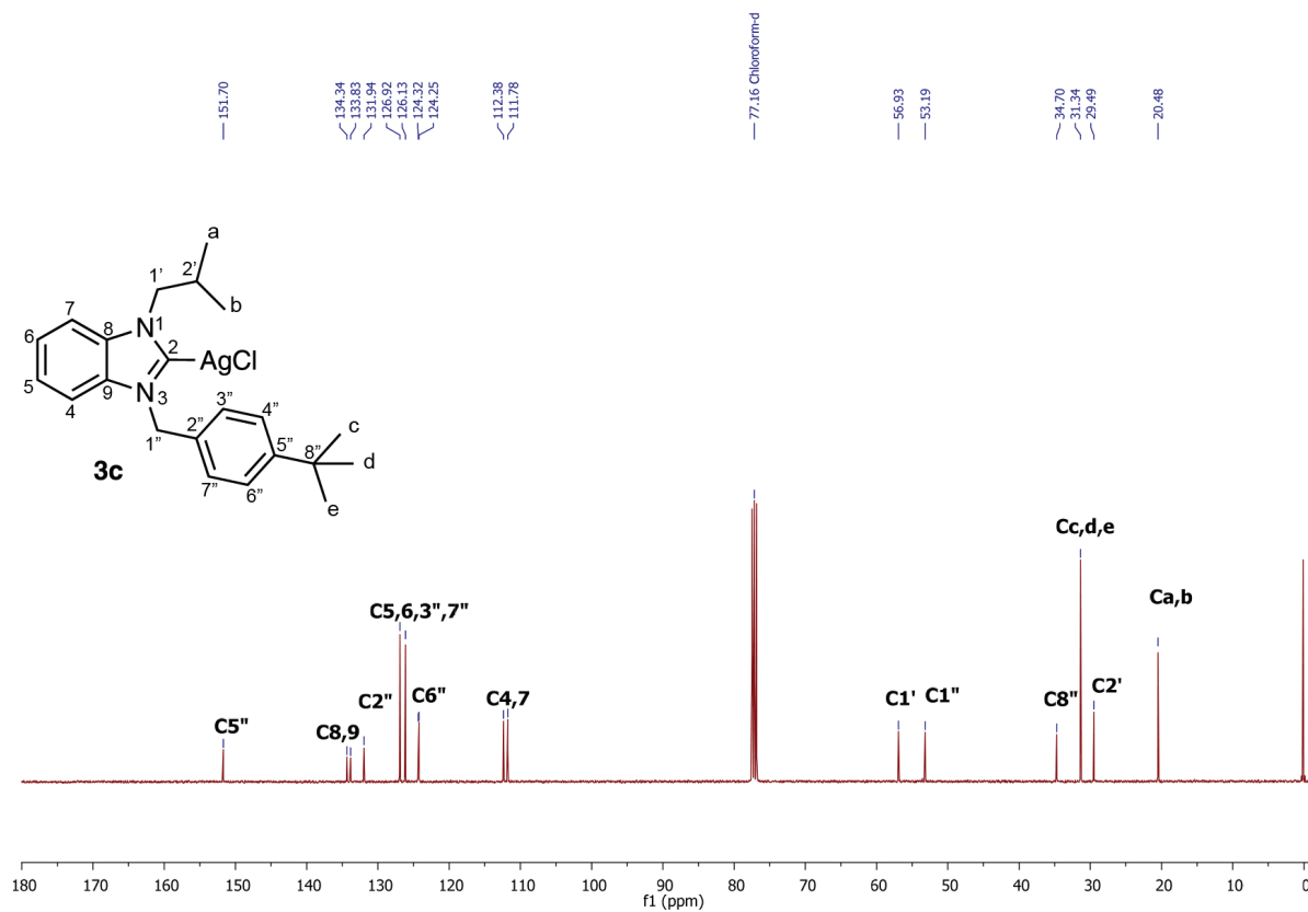
Figure 2. ^{13}\text{C} NMR spectra (100 MHz, \text{CDCl}_3 ) of silver complex 3c .
