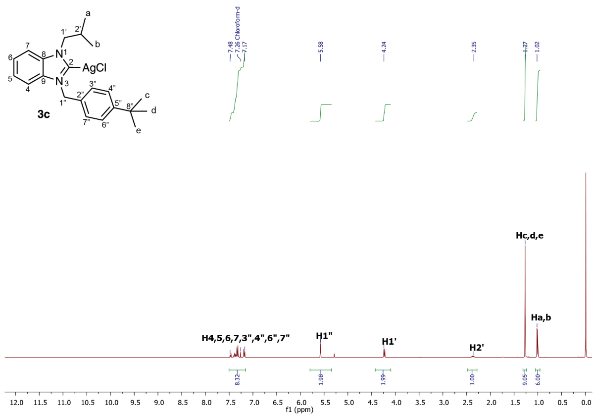
Figure 1. ^1\text{H} NMR spectra (400 MHz, \text{CDCl}_3 ) of silver complex 3c .
