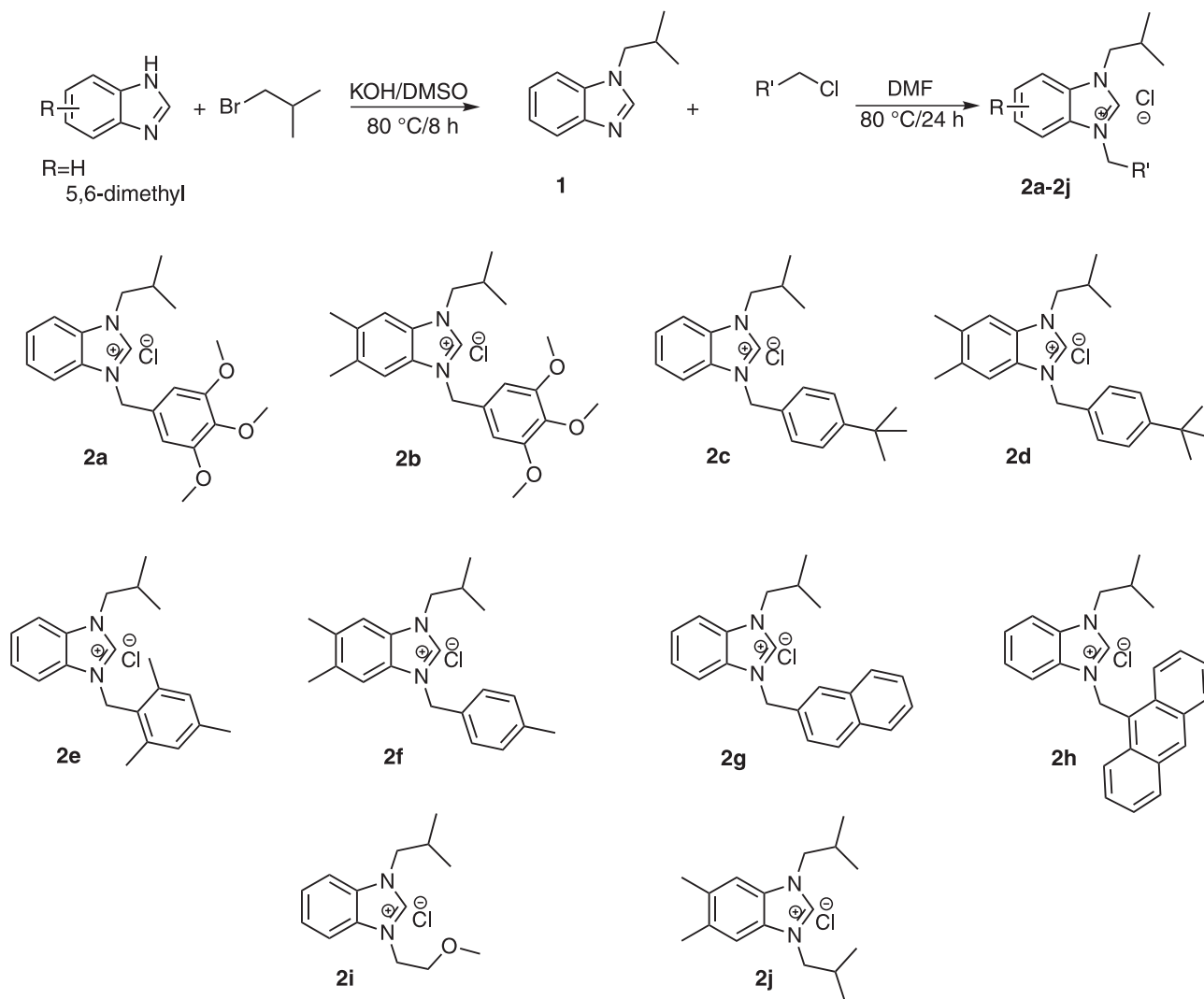
Scheme 1. Synthesis of benzimidazoles salts 2a-2j .
