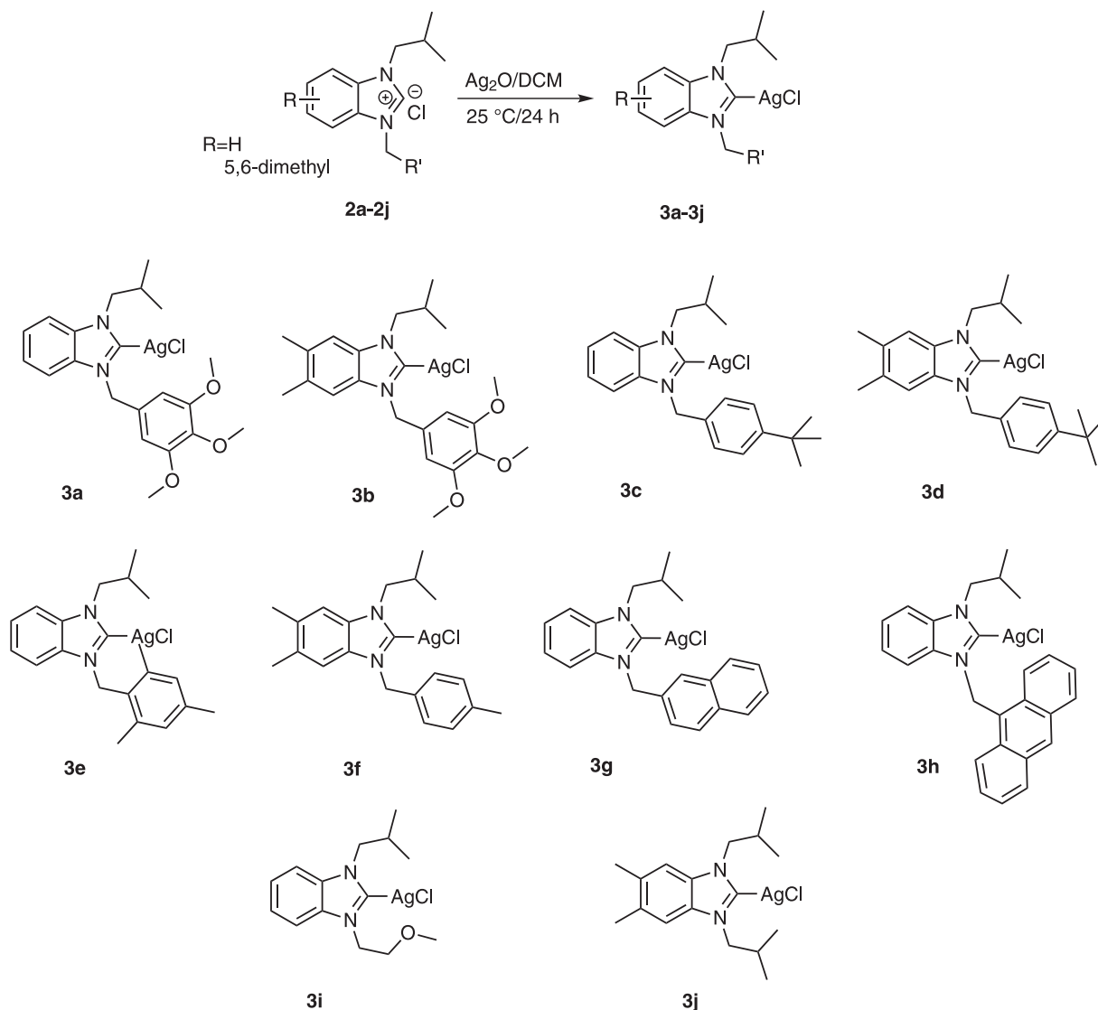
Scheme 2. Protocol synthesis of Ag-NHC 3a-3j .
