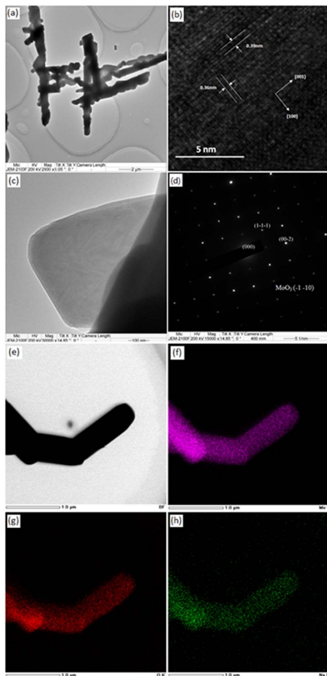
Figure 5 | (a–c) HR-TEM images and (d) SAED patterns of the synthesized \text{Na}_2\text{Mo}_4\text{O}_{13}/\alpha\text{-MoO}_3 hybrid catalyst. (e) TEM image, and elemental (f) Mo mapping, (g) O mapping, and (h) Na mapping of the synthesized \text{Na}_2\text{Mo}_4\text{O}_{13}/\alpha\text{-MoO}_3 hybrid catalyst.
