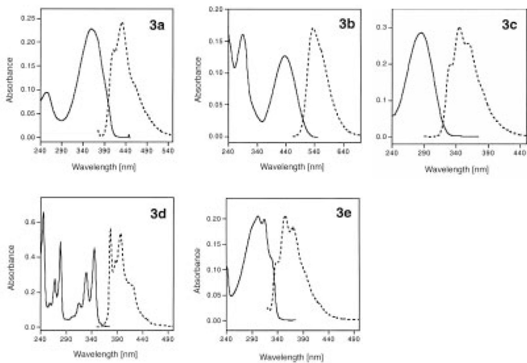
Figure 1. Absorption (—) and normalized emission spectra (- - -) of free nucleosides 3a – e at 10 \mu\text{M} concentration in methanol. Arbitrary intensity units for the emission spectra, with excitation at the absorption maxima.
