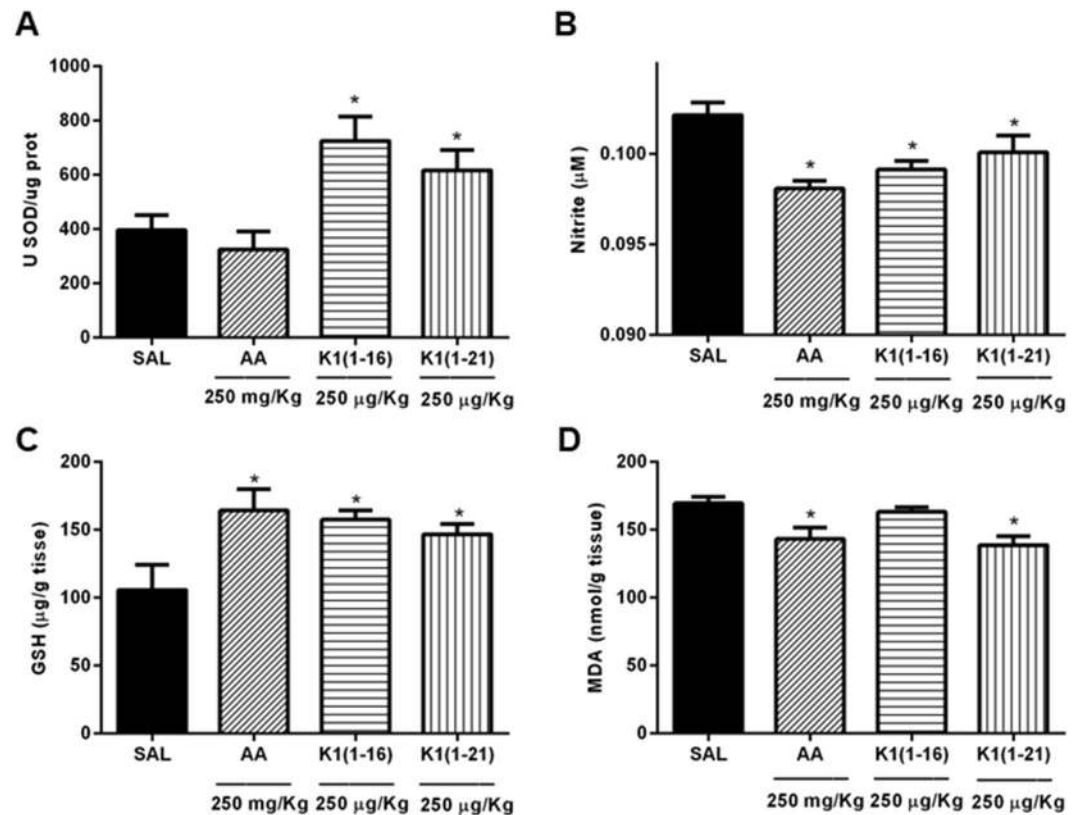
Figure 5. Oxidative parameters in hippocampus of mice acutely treated with Ocellatin-K1(1–16) and Ocellatin-K1(1–21). (A) SOD relative enzymatic activity, (B) nitrite content, (C) GSH, and (D) MDA concentration. Ascorbic acid was used as a standard antioxidant. The results are expressed as mean \pm SEM of a minimum of six animals per group. * p < 0.05 vs. saline group employing ANOVA and Newman–Keuls test. Abbreviations: AA: ascorbic acid; GSH: reduced glutathione; K1(1–16): Ocellatin-K1(1–16); K1(1–21): Ocellatin-K1(1–21); MDA: malondialdehyde; SAL: saline; SOD: superoxide dismutase.
