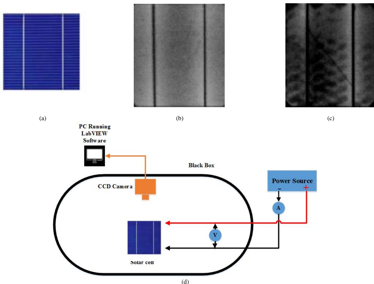
Fig. 1. (a) Ten Examined PV modules, (b) Healthy (crack-free) PV solar cell sample, (c) Cracked PV solar cell sample, (d) Electroluminescence experimental setup
