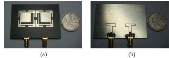
Fig. 15. Photographs of the fabricated CPW-feed dual-mode dual-band Filter III. (a) Top view. (b) Bottom view.
