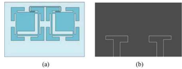
Fig. 14. Configuration of the CPW-feed dual-mode dual-band Filter III. (a) Top view (b) Bottom view. The dimensions are c = 1.5 mm, l_1 = 2.4 mm, l_2 = 12.5 mm, l_3 = 5.3 mm, l_4 = 1.5 mm, l_5 = 3.8 mm, l_6 = 3 mm, l_7 = 0.5 mm, L = 1.2 mm. Other dimensions of CLSLR are the same as Filter I.
