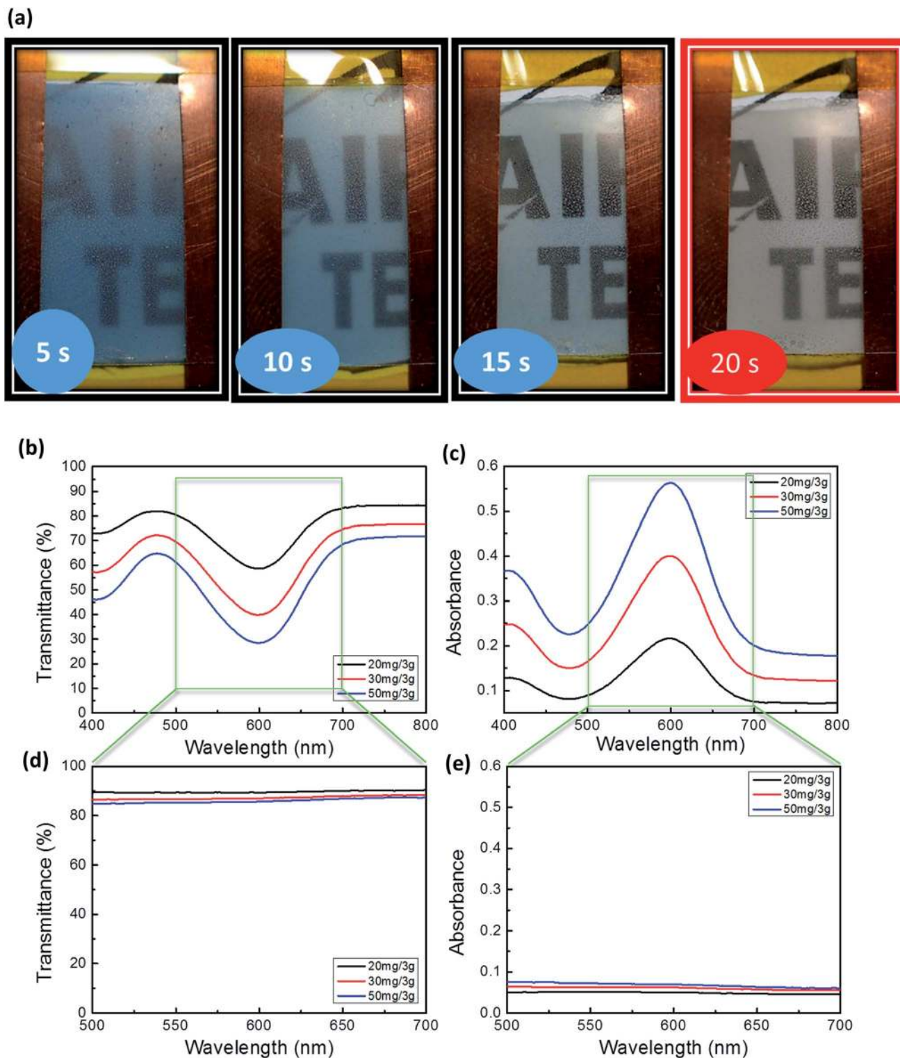
Fig. 4 (a) Thermo-chromic response exhibited by the thermo-chromic ink and silver nanowire-coated polydimethylsiloxane device after the application of 5 V, (b and c) transmittance and absorbance plot of thermo-chromic ink-blended polydimethylsiloxane (TC-PDMS) before applying potential of 5 V, and (d and e) transmittance and absorbance plot of TC-PDMS after applying potential of 5 V.
