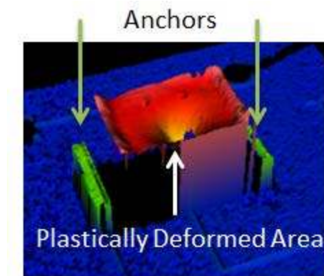
Figure 50 Zygo 3D Image of Fixed-Fixed Au Micro-Contact Support Structure
