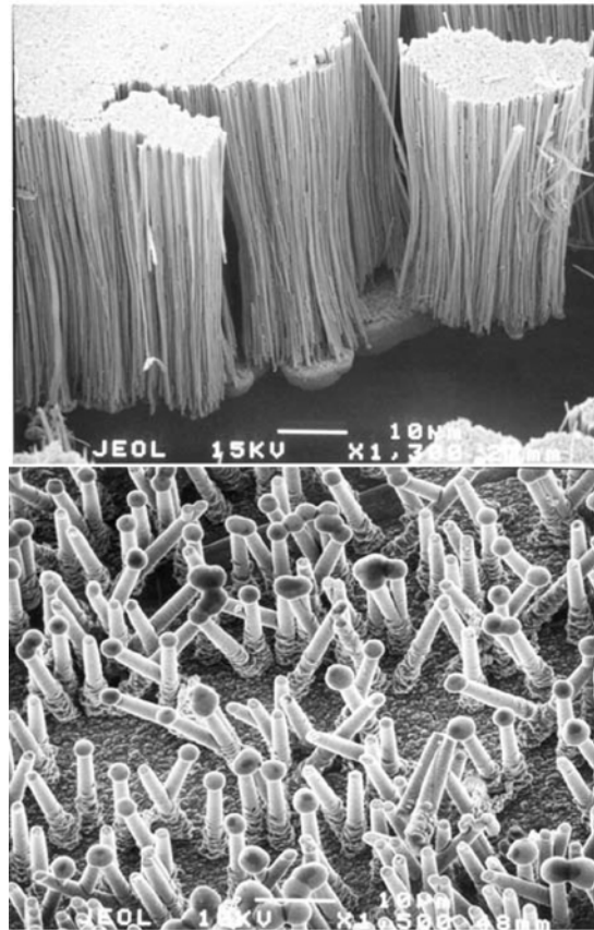
Figure 19 SEM images of nickel nanowires (.2x60 \mu m on top and 2x20 \mu m nickel nanowires with sphere tips) [91]
