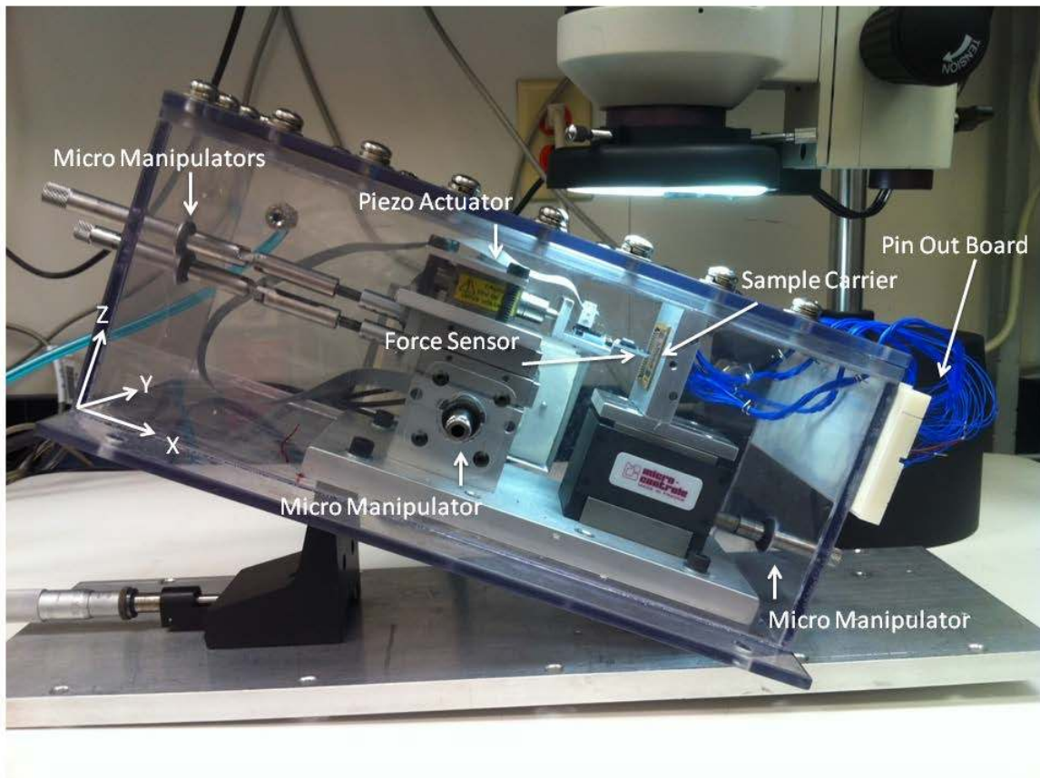
Figure 20 Test Stand
