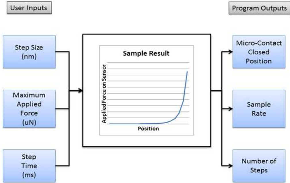
Figure 70 Virgin Contact Test Program Block Diagram
