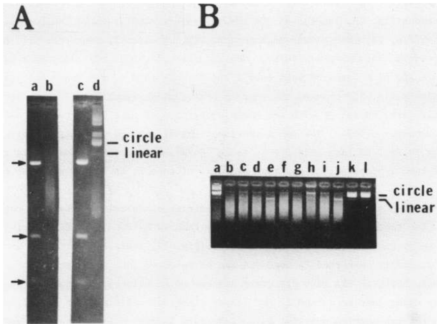
Fig. 2. Gel electrophoretic analysis of the P4 phage DNA and P4 head DNA. (A): P4 head DNA(0.4 \mu g)(b) and P4 phage DNA(0.3 \mu g)(d) were each treated with 2 units of Eco RI restriction endonuclease. Lanes a and c show the restricted products of P4 phage DNA(lane d) and P4 head DNA(lane b) respectively. The arrows indicate the DNA fragments generated by the restriction reaction. Samples were run on a 0.7% agarose gel as described in Materials and Methods. (B): P4 head DNA was treated with various DNA topoisomerases; (a) P4 phage DNA control, (b) P4 head DNA control, (c) head DNA + 0.1 \mu g(22,000 units) of HeLa topo I(100 K form)(13), (d) head DNA + 0.02 \mu g(4,400 units) of HeLa nicking-closing enzyme(67 K form)(13), (e) head DNA + 2 \mu g(5000 units) (24) of E. coli topo I, (f) head DNA + 0.5 \mu g of T4 DNA topoisomerase(19) and (g) head DNA + 0.1 \mu g of HeLa topo II(14). (h)-(l) were repeat of (c)-(g) in the presence of 1 mM ATP. All reactions were treated with 100 \mu g/ml of proteinase K at 30°C for 20 min before loading onto a 0.7% agarose gel.
