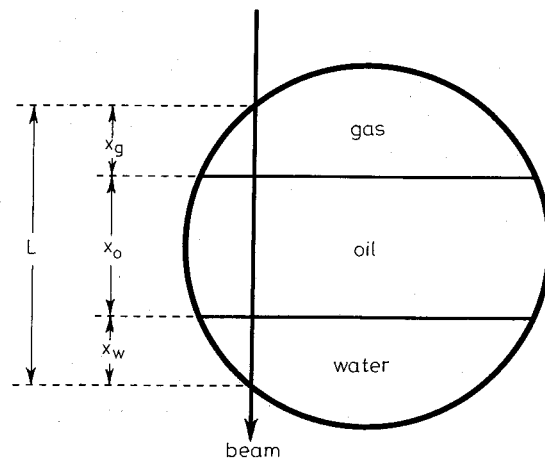
Fig. 3 Gamma beam passing through a pipe containing water, oil and gas in a stratified configuration
